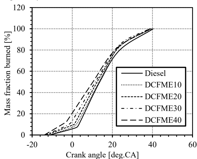
FIGURE 8 Variation of mass fraction burned with crank angle for diesel and DCFME blends.
