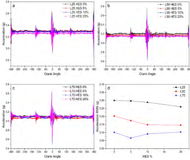
FIGURE 4. Acceleration vs Crank angle variation for (a) 25% load; (b) 50% load; (c) 75% load. (d) RMS value for acceleration at HES values for different loads.
