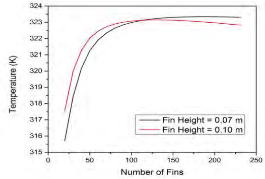
FIGURE 2: VARIATION OF OUTLET TEMPERATURE WITH NUMBER OF FINS FOR FIN THICKNESS t_1 = 0.002 m AND t_2 = 0.001 m.
