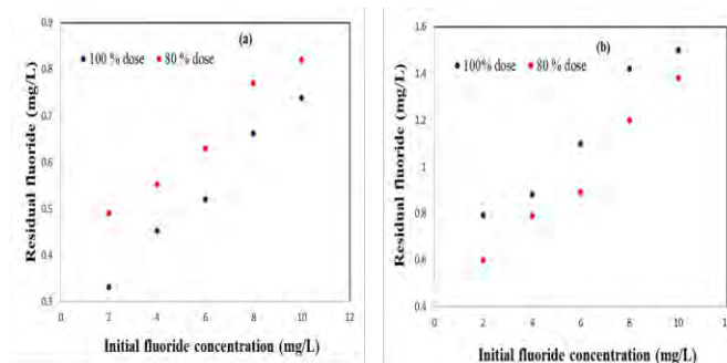
FIGURE 1 Comparative fluoride removal efficiency of (a) alum and (b) PAC at 80% and 100% doses in batch mode
