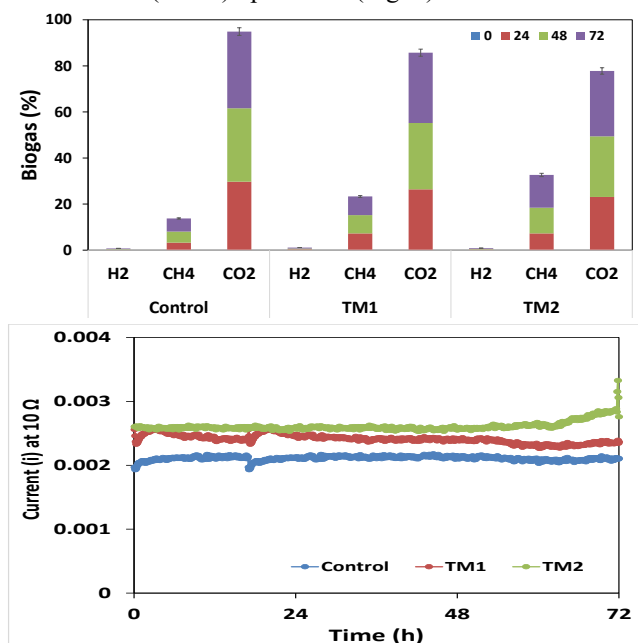
Figure 2. (a) Biogas (%) composition, and (b) Currents profile of MES bioreactor operated at varying trace metal concentrations.
