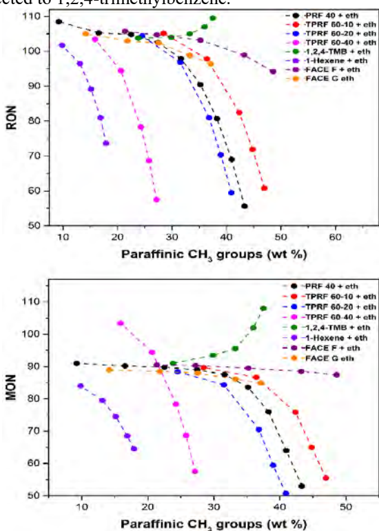
FIGURE 1: Effect of paraffinic CH 3 groups on RON and MON of the blends
