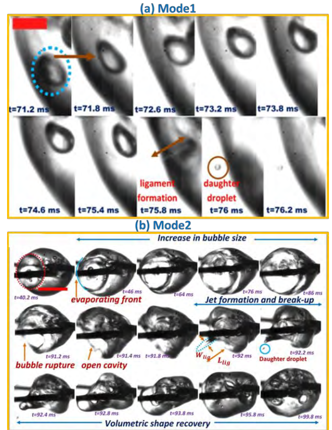
FIGURE 5 (a) High speed images of localised single bubble expulsion from the droplet surface with \alpha_{\text{local}} \sim O(10^{-3})
