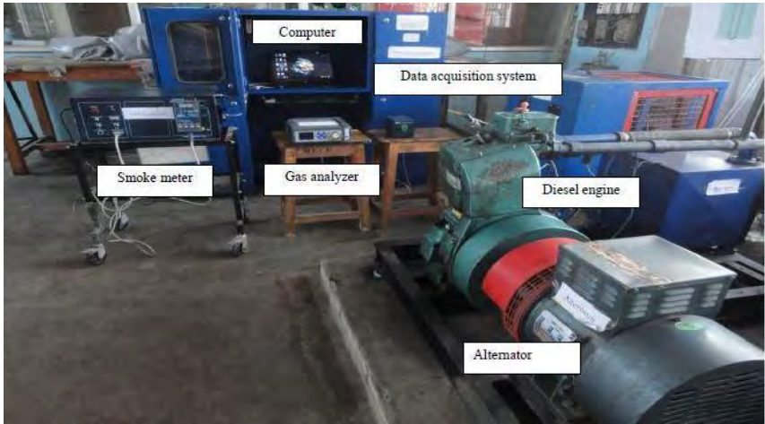
Photograph of the test engine
