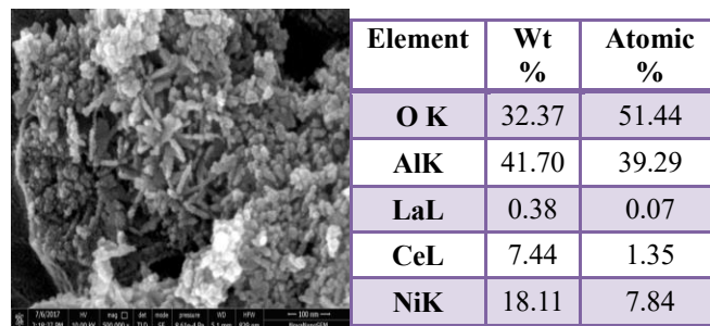
Figure 3 SEM image and EDAX analysis of Ni/ALC
