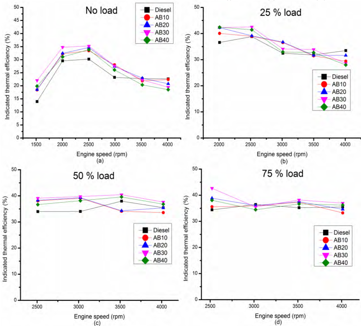
FIGURE 3. INDICATED THERMAL EFFICIENCY
