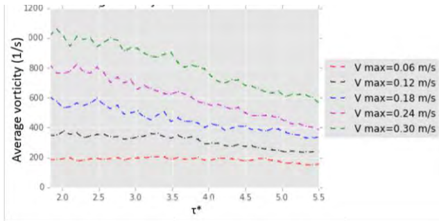
FIGURE 6. Transient variation of average vorticity in a thermal energy storage tank.
