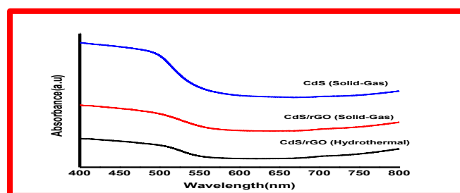
Figure 5 Diffuse reflectance spectra of CdS/rGO(HY), CdS/rGO(SG) and CdS(SG)
