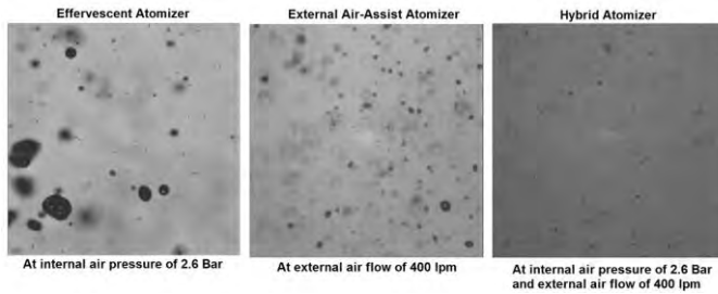
FIGURE 3. Droplet size reduction in three modes
