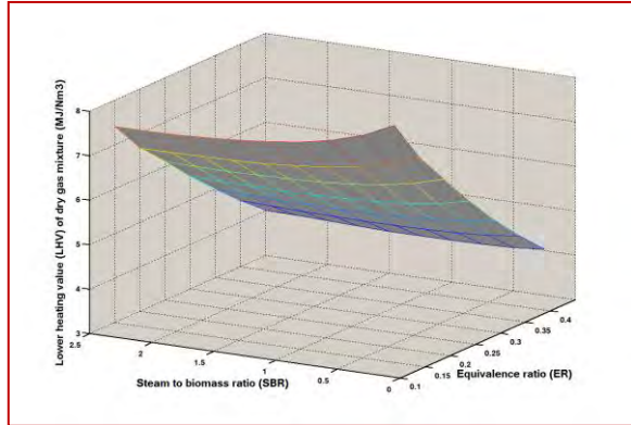
FIGURE 4 VARIATION OF LHV WITH ER AND SBR (T: 1000 K)
