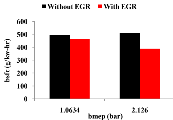
FIGURE 4: COMPARISON OF BSFC WITH AND WITHOUT EGR
