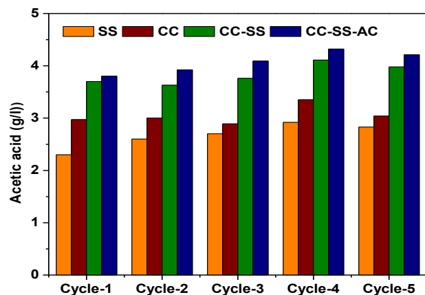
Fig.1 Acetic acid production of all the biocathodes for five cycles of operation
