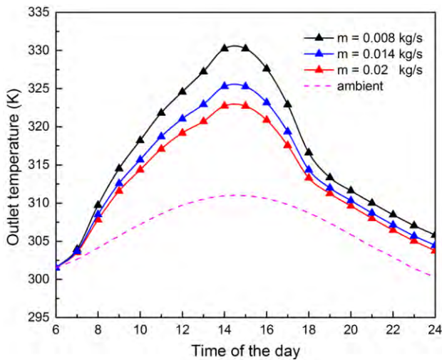
FIGURE 4. TRANSIENT VARIATION OF OUTLET TEMPERATURE FOR VARIOUS MASS FLOW RATES OF AIR (SAH with PCM).
