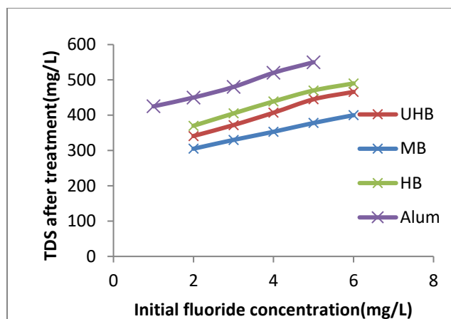
Fig.3: TDS (mg/L) after treatment with Alum and IPC variants
