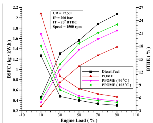
FIGURE 2. Variations of BSFC and BTHE for different test fuels in diesel engine with engine load.
