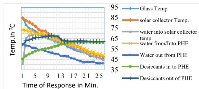
FIGURE 5. SOLAR COLLECTOR TEMPERATURE, WATER TEMPERATURE AND DESICCANT REGENERATED IN PHE.
