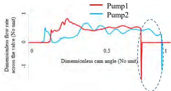
FIGURE 4. DIMENSIONLESS FLOW RATE ACROSS THE INLET VALVE
