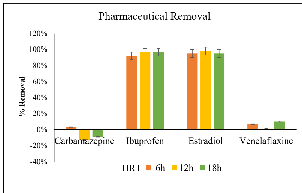
FIGURE 1: REMOVAL OF PHARMACEUTICALS AT VARYING HRT DURATION IN SMBR.
