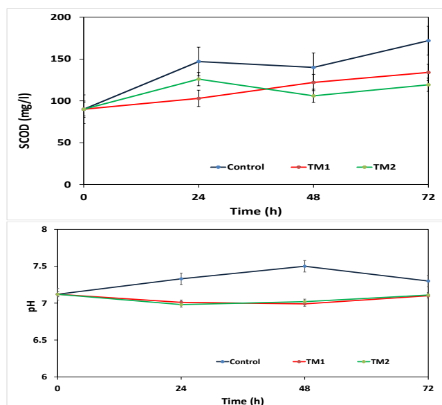
Figure 4. (a) SCOD concentration (mg/l), and (b) pH profiles of MES bioreactor operated at varying trace metal concentrations.
