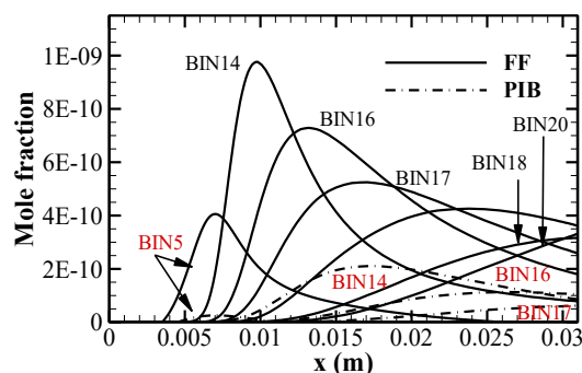
FIGURE 5. BINs concentrations along the flame axis
