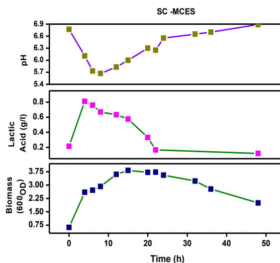
FIGURE 1: The profile specifies pH change, lactic acid production and biomass with respect to time for Closed circuit operation Single chamber MCES.
