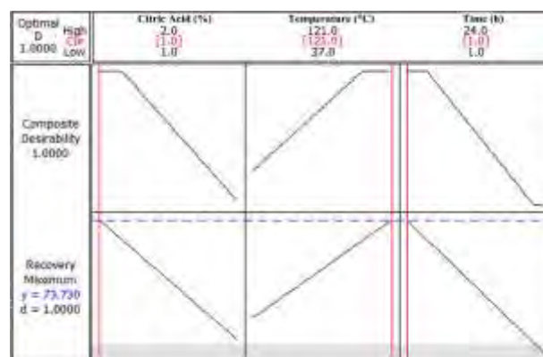
FIGURE 3. RESPONSE OPTIMIZATION PLOT FOR RECOVERY OF CHITIN
