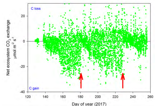
FIGURE 4. Seasonal CO 2 exchange (NEE) from a perennial legume crop in Finland during the 2017 growing season (the red arrows show the days of the year when the crop was harvested).
