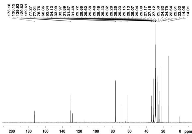
FIGURE 4: 13 C NMR OF BIOSURFACTANT
