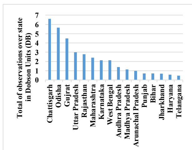
FIGURE 2: (A) FOSSIL FUEL CONSUMPTION IN INDIA, (B) SO 2 INCREASE 2009 TO 2015, (C) NO 2 INCREASE 2009 TO 2015
