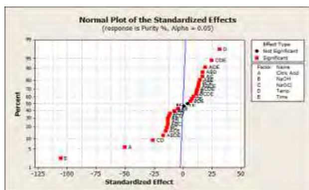
FIGURE 2. NORMAL PLOT FOR PURITY (%) OF CHITIN (R-Sq : 98%)
