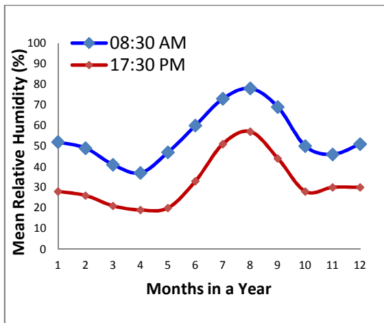
FIGURE 2. PLOT SHOWS MONTHS IN A YEAR VERSUS THE MEAN RELATIVE HUMIDITY IN TWO TIMES AT A DAY TIME IN UTC AT 3 (i.e. 08:30 IST) AND 12 (i.e. 17:30 IST).
