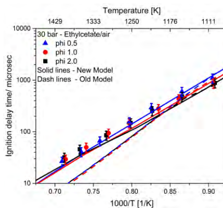
FIGURE 6: COMPARISON OF ETHYL ACETATE IGNITION DELAY DATA WITH PROPOSED MODEL AND MODEL BY WESTBROOK ET AL.
