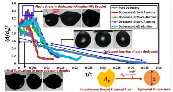
FIGURE 4 Temporal variation of the normalised droplet diameter showing linear regression for pure dodecane and heightened fluctuations for nanofuel droplets. Droplet lifetime is normalised by the thermal diffusive time scale \tau .
