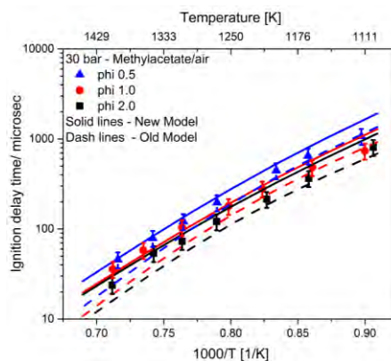
FIGURE 4: COMPARISON OF METHYL ACETATE IGNITION DELAY DATA WITH PROPOSED MODEL AND MODEL BY WESTBROOK ET AL.
