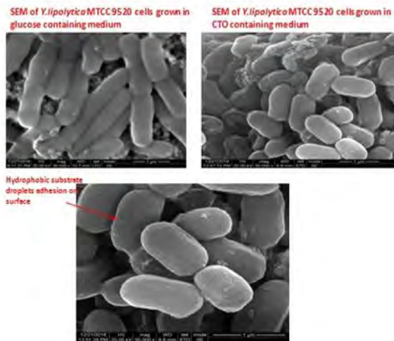
FIGURE 2. SCANNING ELECTRON MICROSCOPY ANALYSIS OF YARROWIA LIPOLYTICA MTCC 9520
