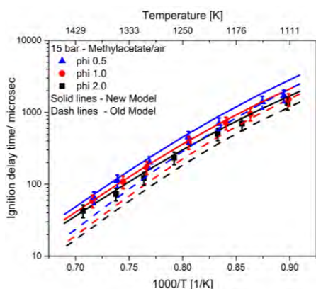
FIGURE 3: COMPARISON OF METHYL ACETATE IGNITION DELAY DATA WITH PROPOSED MODEL AND MODEL BY WESTBROOK ET AL.
