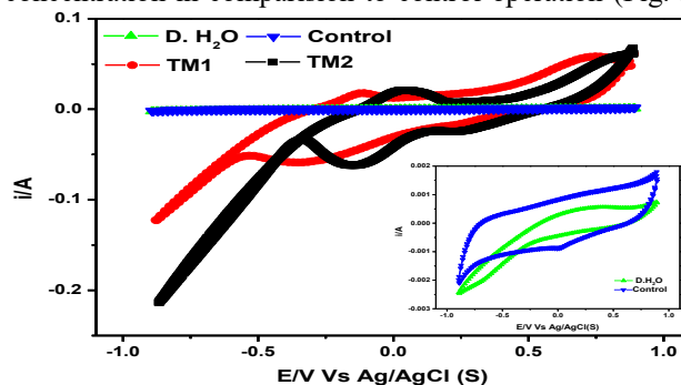
Figure 3. Cyclic voltammetric profiles with respect to control and 2 different concentrations of trace metals
