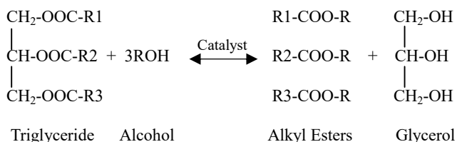
FIGURE 2. TRANSESTERIFICATION REACTION
