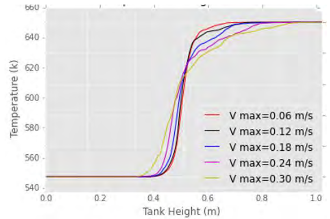
FIGURE 4. Axial distribution of temperature at 60s across all five cases
