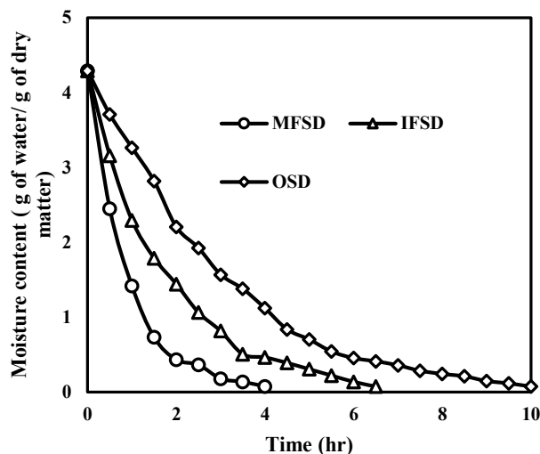
FIG.5.VARIATION OF MOISTURE CONTENT ON DRYBASIS WITH TIME
