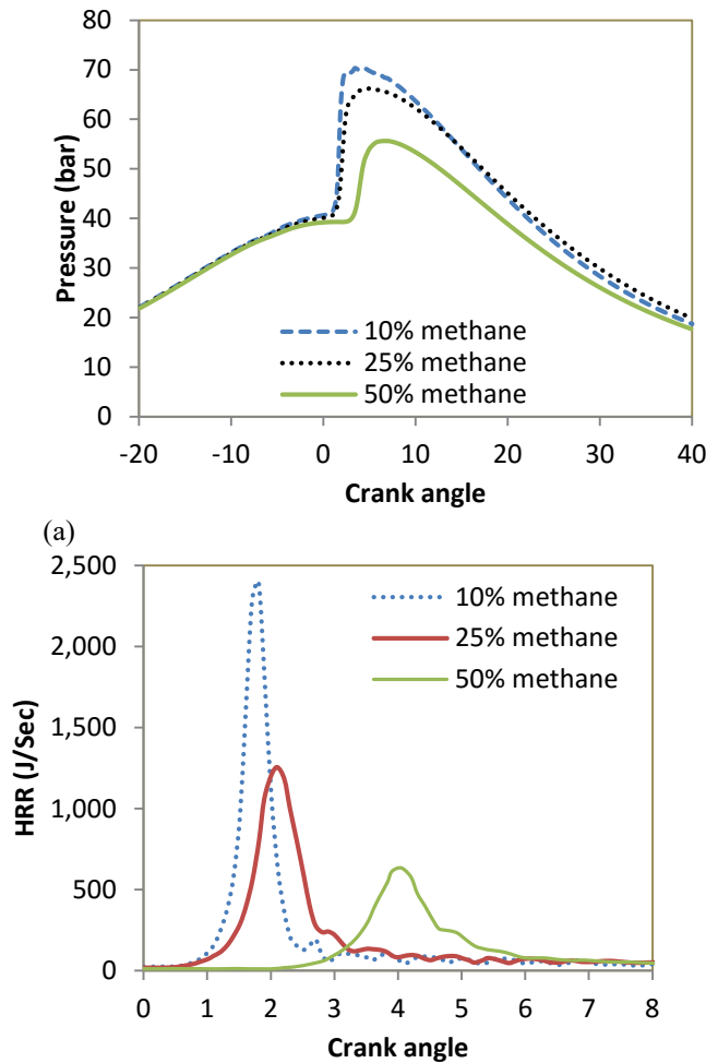
FIGURE 2. (a) COMPARISON OF PRESSURE FOR VARYING METHANE PERCENTAGE AND (b) HRR VARIATION WITH METHANE PERCENTAGE
