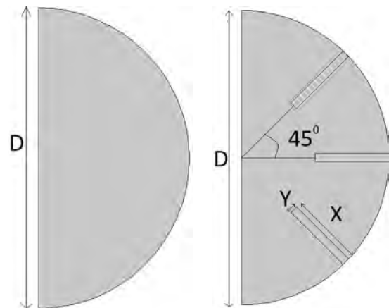
FIGURE 2. MODEL A) UNFINNED B) FINNED
