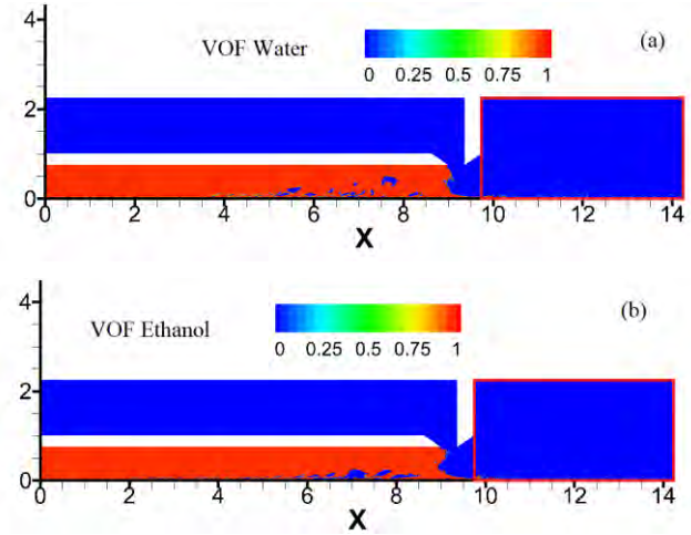
FIGURE 4. CONTOUR OF VOLUME OF FLUID
