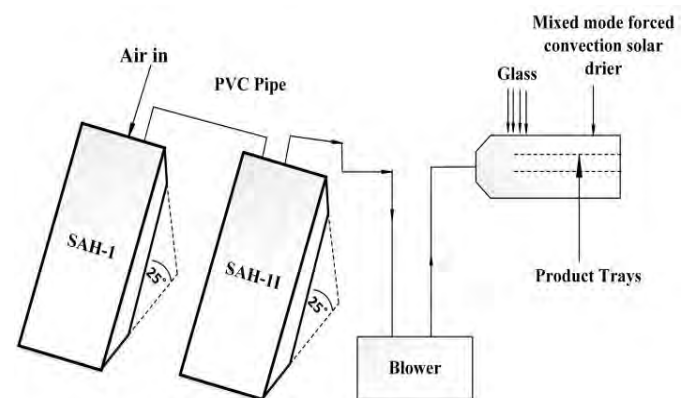
FIG.1: SCHEMATIC OF MIXED MODE FORCED CONVECTION SOLAR DRYER
