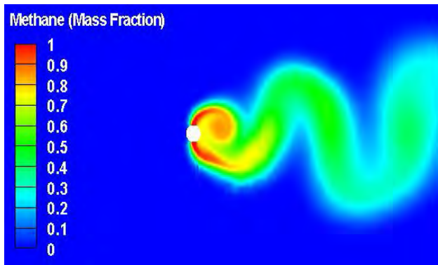
Fig. 6: Methane mole fraction contours for \phi=1
