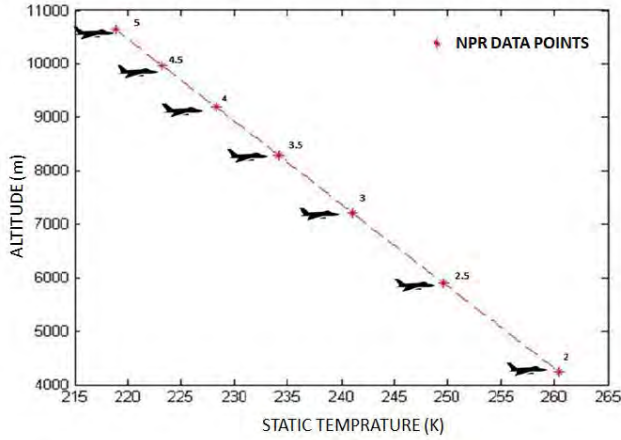
FIGURE 2. CHANGE IN NPR WITH ALTITUDE
