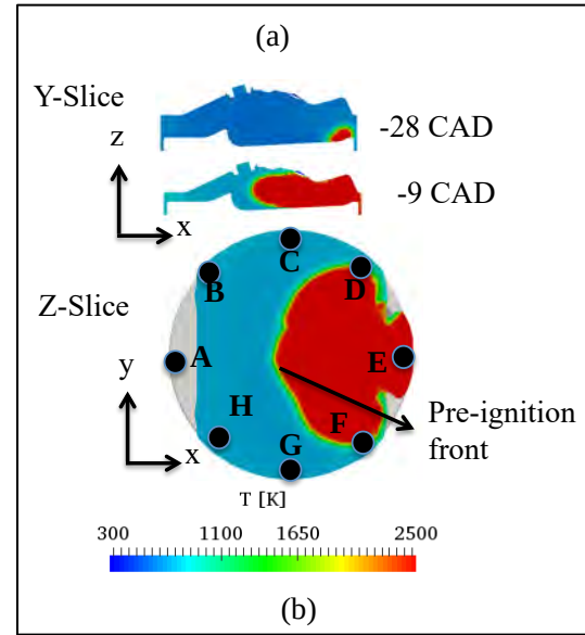
FIGURE 2: (a) Y-SLICE SHOWING HOTSPOT AND PRE-IGNITION FLAME FRONT, (b) LOCATIONS OF POINT A-F SELECTED FOR ANALYSIS.
