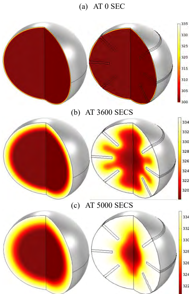
FIGURE 4. TEMPERATURES CONTOUR (K) FOR A) UNFINNED B) FINNED PCM CAPSULE AT (A) 0, (B) 3600, (C) 5000 SECONDS OF THE CHARGING TEST WITH CONSTANT TEMPERATURE WALL TEMPERATURE.
