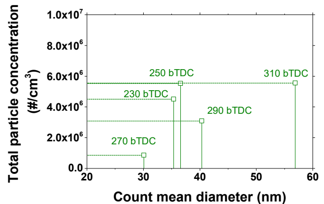
Figure 5: Co-relation between total particle concentration and count mean diameter
