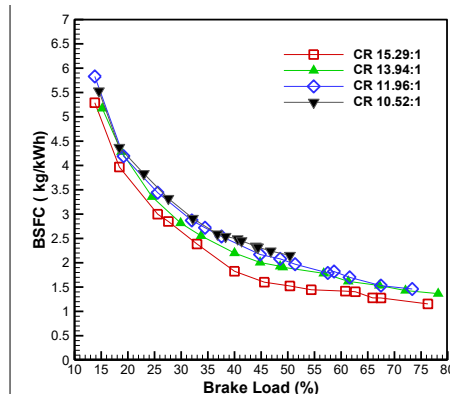
FIGURE 4. BRAKE SPECIFIC FUEL CONSUMPTION OF THE ENGINE AT DIFFERENT CR
