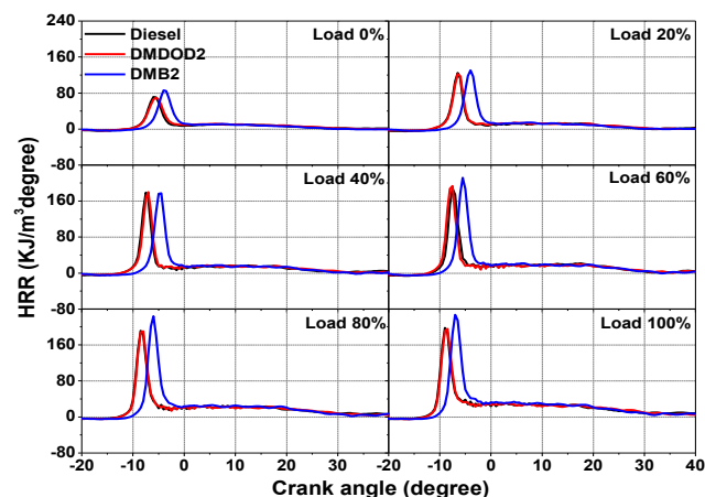
Figure 4. HRR variation with CAD and engine load
