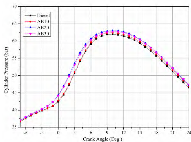
FIGURE 1. Cylinder pressure vs. Crank angle
