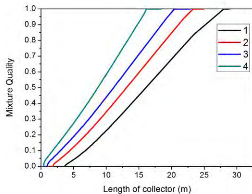
FIGURE 5. MIXTURE QUALITY VS TUBE LENGTH FOR DIFFERENT MIXTURE
