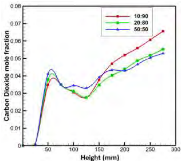
Figure 7c: Variation in mole fraction of carbon dioxide along the height of cook stove
