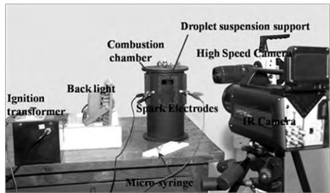
Figure-1 Droplet combustion experimental setup
