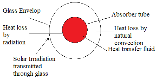
Figure 2. Schematic diagram of evacuated receiver
