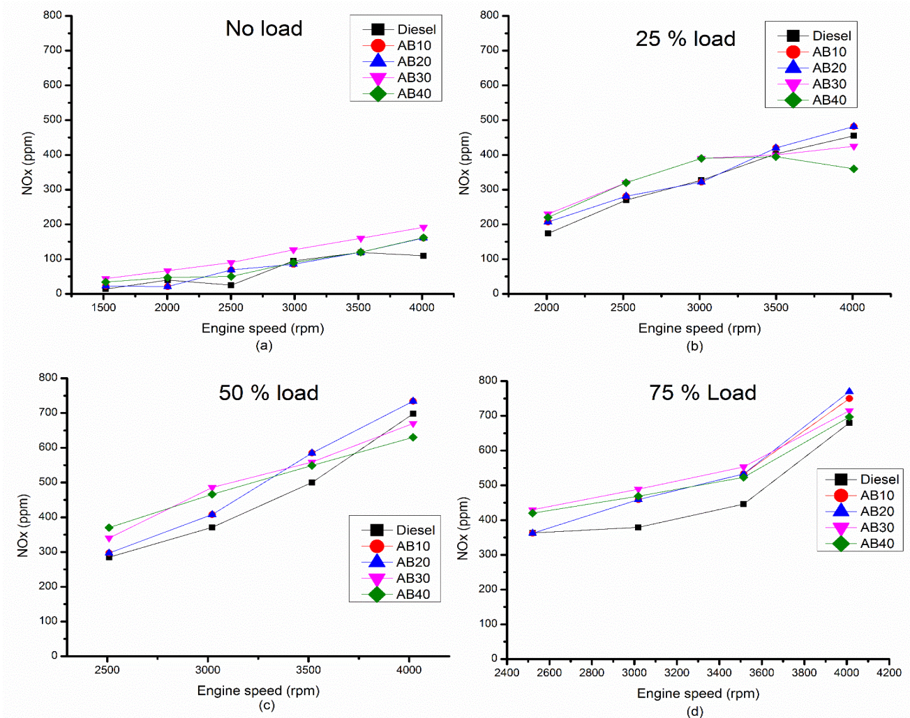
FIGURE 5. NO x VARIATION OF VARIOUS BLENDS WITH DIFFERENT ENGINE LOAD AND SPEED (RPM)
