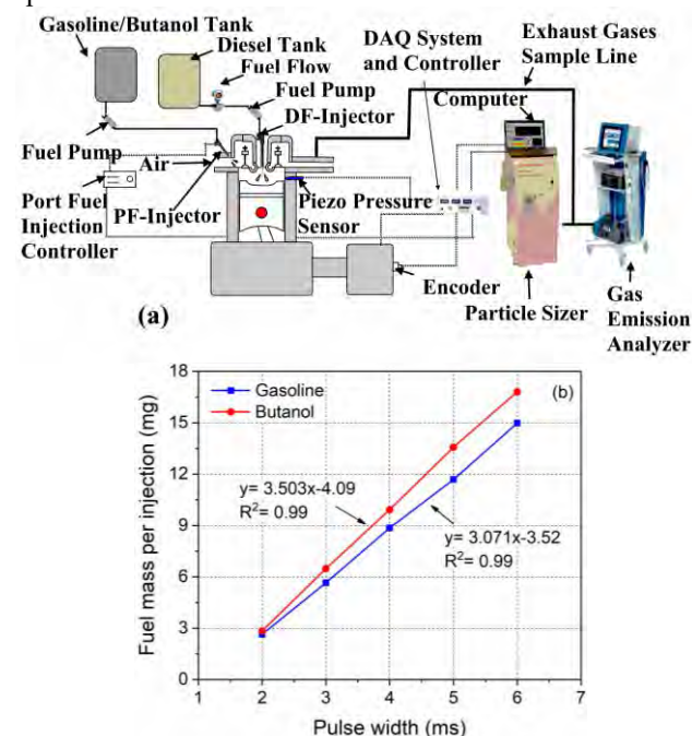
FIGURE 1. (a) Schematic diagram of experimental setup (b) Calibration curve for port injector of gasoline and butanol
