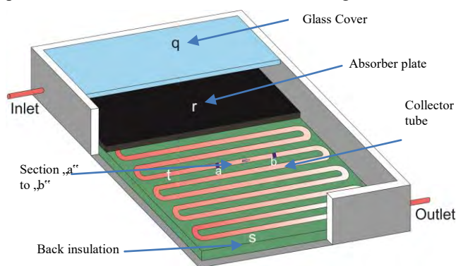
FIGURE 1. SCHEMATIC OF SERPENTINE TUBE FLAT PLATE SOLAR COLLECTOR
