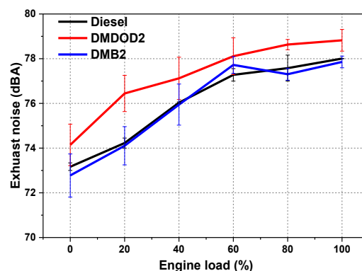
Figure 6. Variation of exhaust noise with engine loads
