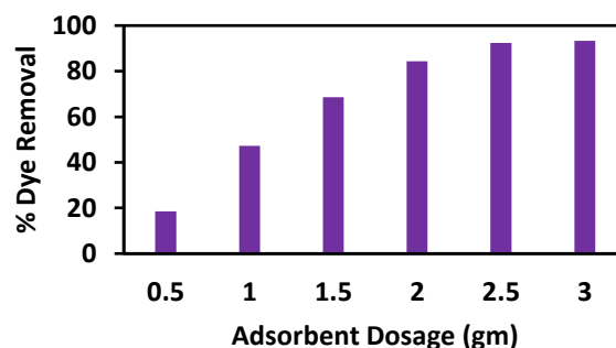
FIGURE 3. THE EFFECT OF ADSORBENT DOSAGES ON THE DECOLORIZATION OF ACID RED 3BN. (CONDITIONS: INITIAL DYE CONCENTRATION 100 PPM; AGITATION SPEE= 100 RPM; TIME = 240 min; CONTACT PH 7; DOSAGE OF ADSORBENT = 2.5 gm = VARIABLE).
