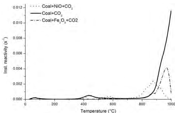
FIGURE 2. Instantaneous reactivity of low ash coal with \text{Fe}_2\text{O}_3 and \text{NiO} in \text{CO}_2 atmosphere
