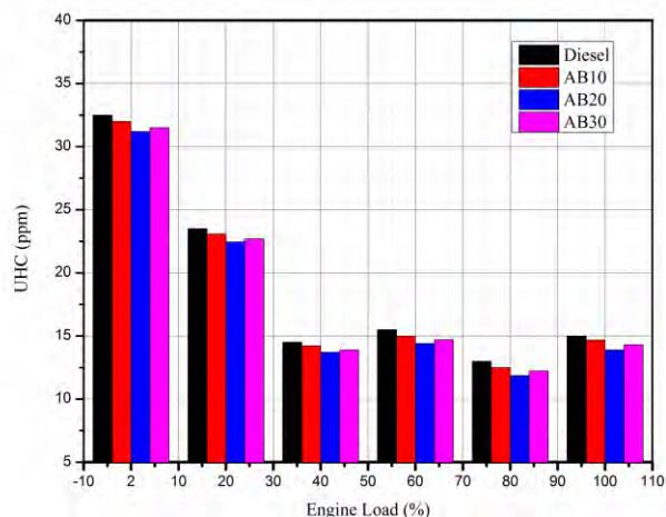
FIGURE 7. UHC vs. engine load
