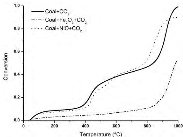
FIGURE 4. Conversion of \text{NiO} -coal and \text{Fe}_2\text{O}_3 -coal mixture in \text{CO}_2 atmosphere
