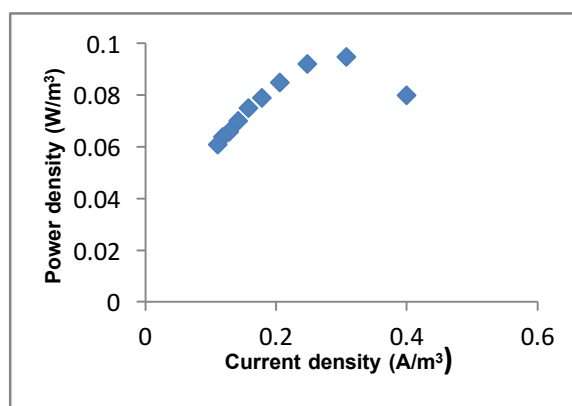
Fig.1.2 POWER GRAPH OF MFC WITH CE
