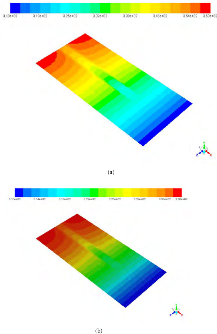
FIGURE 3: Temperature (K) contour at the Ground
