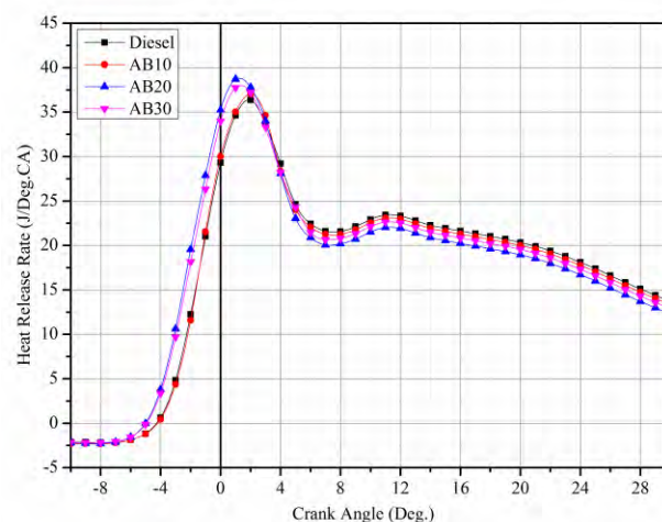
FIGURE 2. Heat release rate vs. Crank angle
