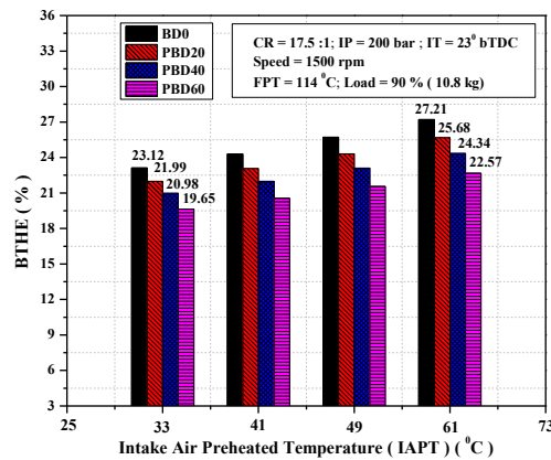
FIGURE 4. Variations of BTHE for different test fuels in diesel engine with intake air preheating temperature.
