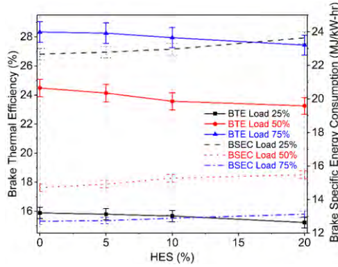
Figure 2 Effect of HES on BTE and BSEC.
