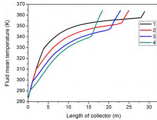
FIGURE 2. FLUID MEAN TEMPERATURE ALONG THE LENGTH OF THE COLLECTOR FOR DIFFERENT REFRIGERANT MIXTURES
