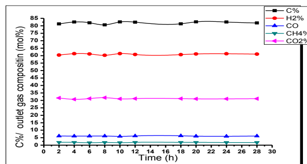
Fig. 6 stability test of 15Ni/ALC at 600 °C
