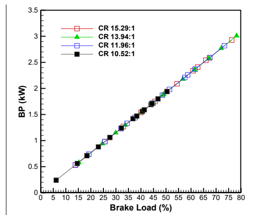
FIGURE 2. BRAKE POWER DEVELOPED BY THE ENGINE ON DIFFERENT COMPRESSION RATIOS
