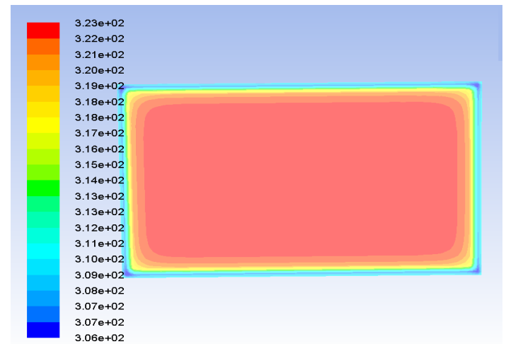
Figure 1: Thermal profile of a PV module at a wind speed of 2 m/s
