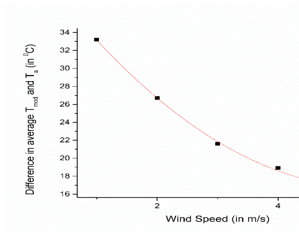
Figure 2: Temperature differential as a function of wind speed
