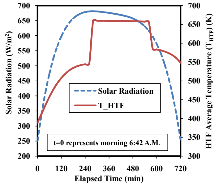
FIGURE 3. Variation of temperature of the heat transfer fluid Duratherm FG ( T_{HTF} ) with the changing solar radiation power ( \bar{P} )
