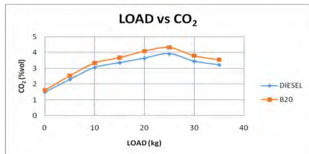
FIGURE 8. LOAD VERSES CARBON DIOXIDE EMISSION
