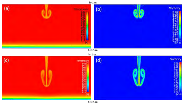
FIGURE 1. Growth of flow disturbance in the form of (a) temperature and (b) vorticity contours at \tau^* = 0.45 ; and (c) temperature and (d) vorticity at \tau^* = 0.82 for case 1.
