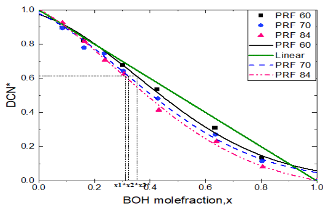
Figure 1: DCN* vs Butan-1-ol (BOH) mole-fraction for PRF 60, PRF 70 and PRF 84. The scattered points, Gaussian fitting
