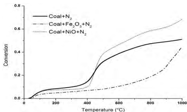
FIGURE 3. Conversion of \text{NiO} -coal and \text{Fe}_2\text{O}_3 -coal mixture in \text{N}_2 atmosphere
