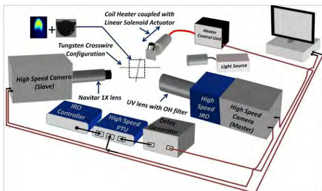
FIGURE 1 Schematic of the experimental setup comprising of high speed camera and chemiluminescence imaging systems for simultaneous capture of droplet shape and flame. Both imaging systems are synced with a droplet ignition apparatus. [6].
