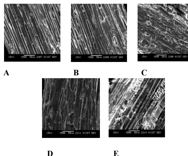
Fig.2. Scanning electron micrographs of native and pretreated samples (A-Native, B-Hydrothermal, C- Nitric acid, D- Lime and E-integrated dilute acid-lime)
