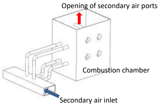
Figure 1b: Internal view of cook stove
