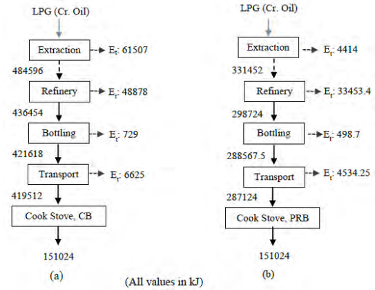
FIGURE 1. ENERGY FLOW DIAGRAM AT 10 kW INPUT POWER
