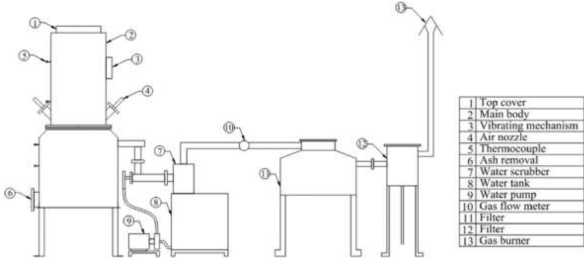
FIGURE 1. SCHEMATIC DIAGRAM OF THE 10 KWE DOWNDRAFT GASIFIER SYSTEM
