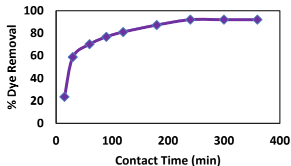
FIGURE 1. THE EFFECT OF CONTACT TIME ON THE DECOLORIZATION OF ACID RED 3BN. (CONDITIONS: INITIAL DYE CONCENTRATION 100 PPM; DOSAGE PH 7; AGITATION SPEE= 100 RPM; OF ADSORBENT = 2.5 gm; CONTACT TIME = VARIABLE).
