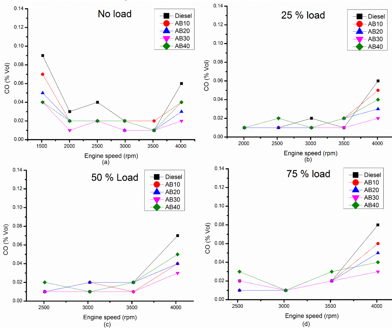
FIGURE 6. CO VARIATION OF VARIOUS BLENDS WITH DIFFERENT ENGINE LOAD AND SPEED (RPM)
