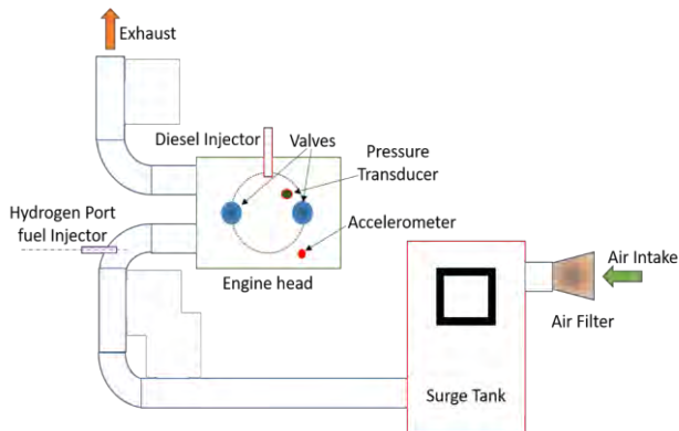
FIGURE 1. Schematic diagram of the test setup.
