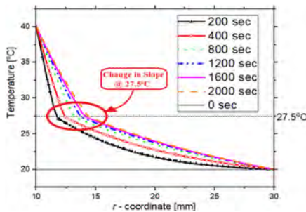
Figure 7. Temperature distribution of PCM (Cylindrical coordinates) - Case 2.
