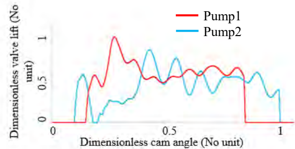
FIGURE 3. DIMENSIONLESS LIFT OF THE INLET VALVE
