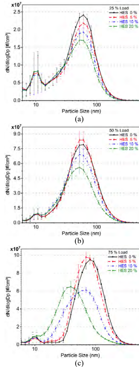
Figure 4 Effect of HES on Particle size distribution at engine loads (a) 25%, (b) 50% and (c) 75 %.
