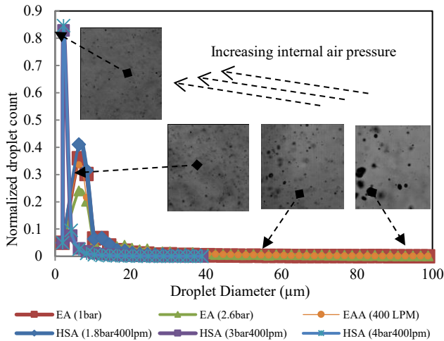
FIGURE 2. Normalized droplet count vs Droplet diameter with increasing internal air pressure
