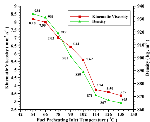
FIGURE 1. Variations of kinematic viscosity and density of POME with fuel inlet preheating temperature.
