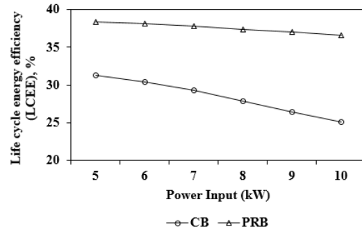
FIGURE 2. VARIATION OF LCEE WITH INPUT POWER
