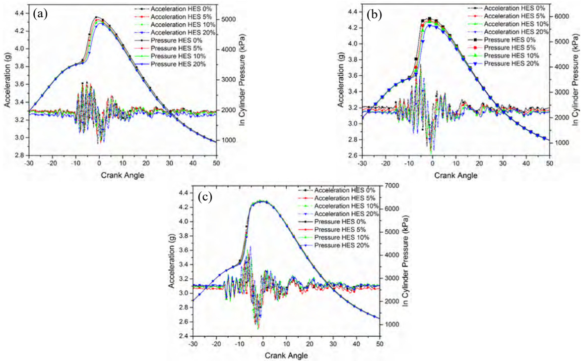
FIGURE 5. In-cylinder pressure variation and engine acceleration plotted against zoomed crank angle degrees for (a) Load 25%; (b) Load 50% and (c) Load 75%.
