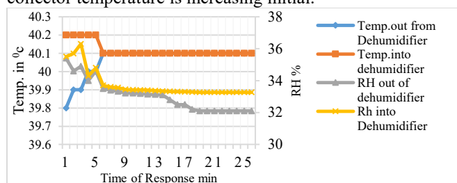
FIGURE6. RELATIVE HUMIDITY AND TEMPERATURE DISTRIBUTION IN DEHUMIDIFIER.
