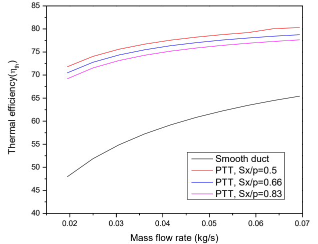
FIG. 3 THERMAL EFFICIENCY AS A FUNCTION OF MASS FLOW RATE.
