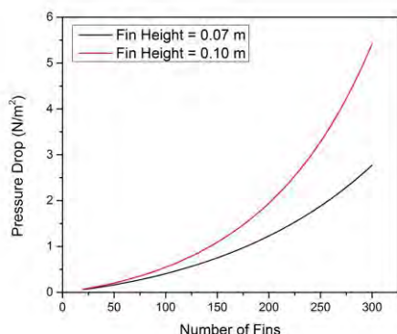
FIGURE 5: PRESSURE DROP V/S NUMBER OF FINS FOR FIN THICKNESS t_1=0.002 m AND t_2=0.001 m.
