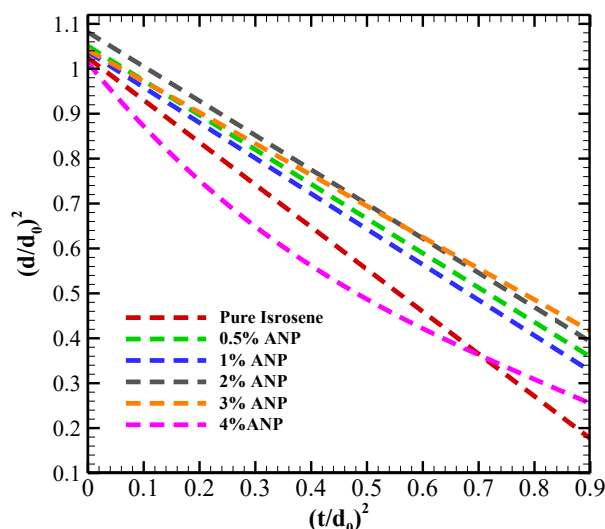
Figure-4 D^2 -t curve for Isrosene and ANP loaded Isrosene droplets
