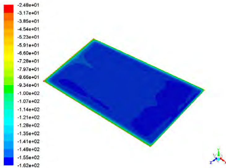
FIGURE 7: Radiative heat flux ( \text{W/m}^2 ) at the layer of Tedlar in PV Module
