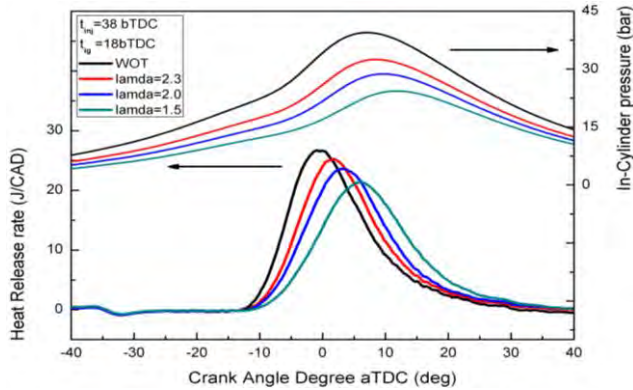
FIGURE 1. HEAT RELEASE AND IN-CYLINDER PRESSURE WITH DIFFERENT AIR-EXCESS RATIO
