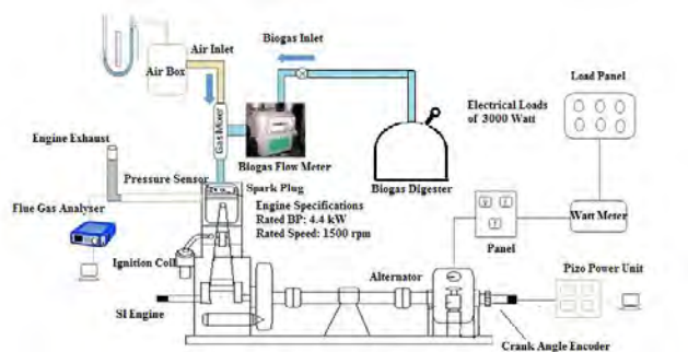
FIGURE 1. SCHEMATIC LAYOUT OF EXPERIMENTAL TEST RIG
