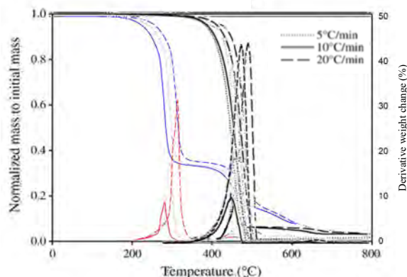
Figure 1. TG and DTG graphs of PE and PVC
