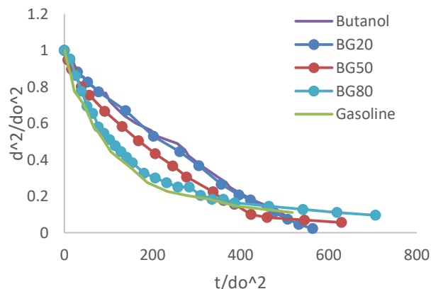
FIGURE 4. Evaporation Behaviour of Butanol Gasoline Blends
