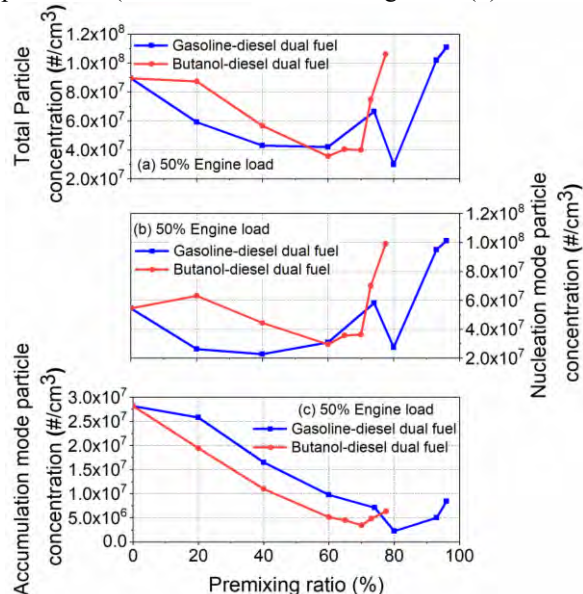
FIGURE 5. Variation of (a) total particle number; (b) nucleation mode; (c) accumulation mode particles concentration with fuel premixing ratio
