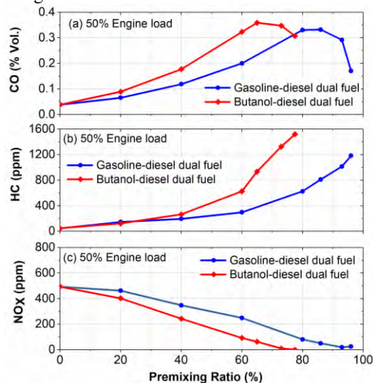
FIGURE 4. Variation of CO, HC, and NO x emission with gasoline/butanol-diesel premixing ratio
