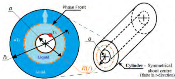
Figure 3. Schematic for cylindrical problem case 2.
