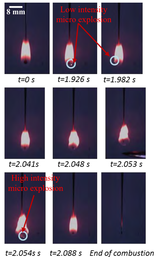
Figure-3 Unsteady flame and presence of low and high intensity micro explosion during the combustion of nanofluid droplet
