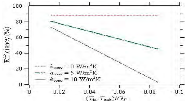
Figure 7 Collector efficiency as a function of temperature difference (for various convective heat transfer coefficients).
