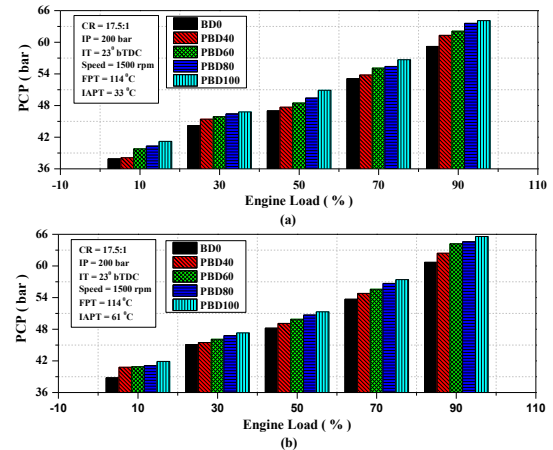
FIGURE 5. Variations of PCP for test fuels in a diesel engine with load with and without intake air preheating.
