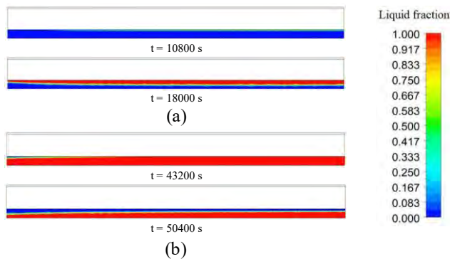
FIGURE 3. LIQUID FRACTION CONTOURS DURING MELTING AND SOLIDIFICATION FOR m = 0.02 kg/s.
