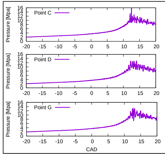
FIGURE 3: IN-CYLINDER LOCAL PRESSURE AT POINTS C, D AND G.
