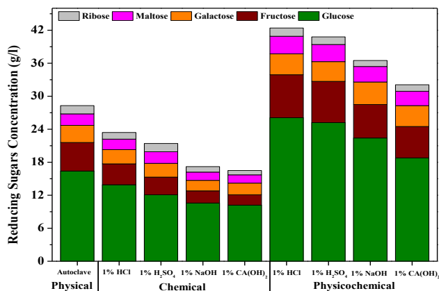
Fig 1: Reducing sugars composition with respect to method of pretreatment
