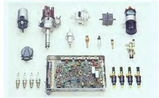
FIGURE 5. D Jetronic components
