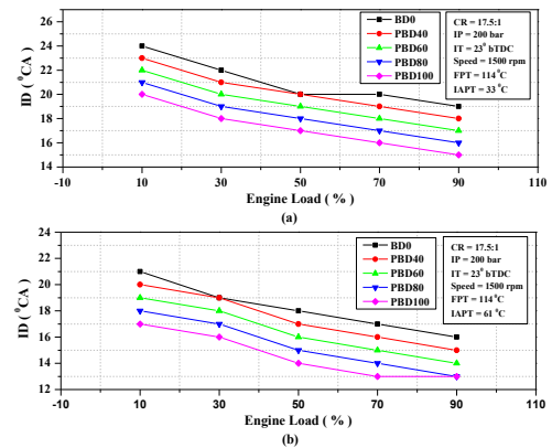
FIGURE 6. Variations of ID for test fuels in a diesel engine with load with and without intake air preheating.
