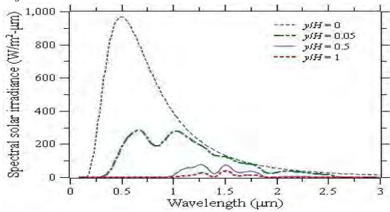
Figure 4 Spectral solar irradiance within the collector at various depths.
