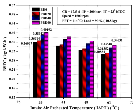
FIGURE 3. Variations of BSFC for different test fuels in diesel engine with intake air preheating temperature.
