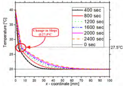
Figure 6. Temperature distribution for PCM (Cartesian coordinates) - Case 2.
