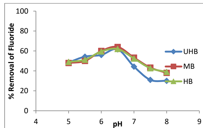
Fig.1: Effect of pH on de-fluoridation efficiency of IPC variants
