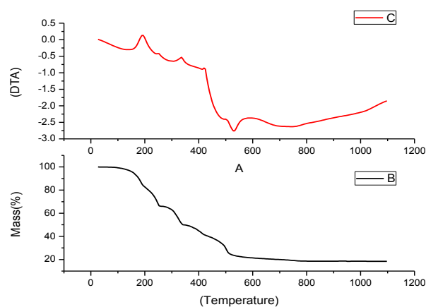
Figure. 1 TG and DTA curves of bis(bipyridine)nickel(II) chloride
