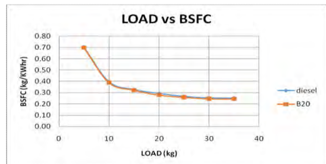
FIGURE 5. LOAD VERSES BRAKE SPECIFIC FUEL CONSUMPTION
