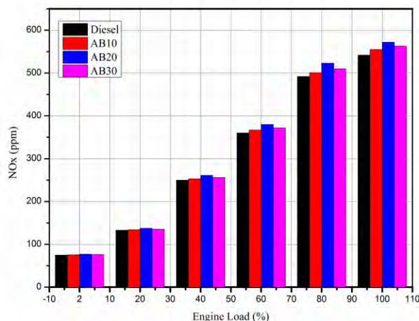
FIGURE 8. Oxide of nitrogen vs. engine load
