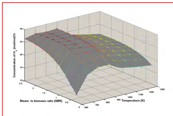
FIGURE 2. VARIATION OF H_2 CONCENTRATION WITH T AND SBR ( ER=0.25 )
