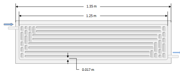
FIGURE .6 MARQUISE SHAPED CHANNEL FLAT PLATE SOLAR COLLECTOR.
