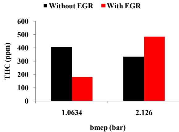
FIGURE 6: COMPARISON OF THC EMISSIONS WITH AND WITHOUT EGR
