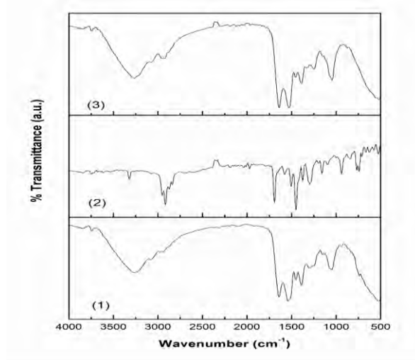
FIGURE 2: ATR-FTIR SPECTRA OF (1) DICNa (2) SER-MODIFIED MEMBRANE AND (3) SER-MODIFIED MEMBRANE AFTER FILTRATION
