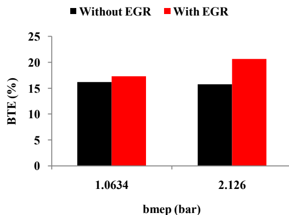
FIGURE 5: COMPARISON OF BTE WITH AND WITHOUT EGR
