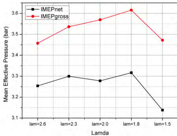
FIGURE 2. MAXIMUM IMEP & GMEP IN EACH CASE
