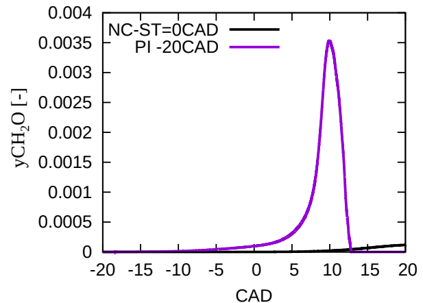
FIGURE 6: COMPARISON OF FORMALDEHYDE FORMATION BETWEEN NORMAL COMBUSTION AND PRE-IGNITION CYCLE.
