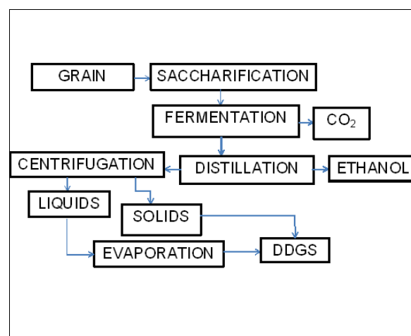
FIGURE 1. FLOW DIAGRAM OF PRODUCTION OF ETHANOL AND IT'S BY PRODUCTS
