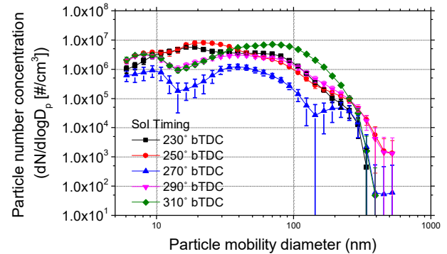
Figure 2: Particle number size distribution vs particle mobility diameter (nm)
