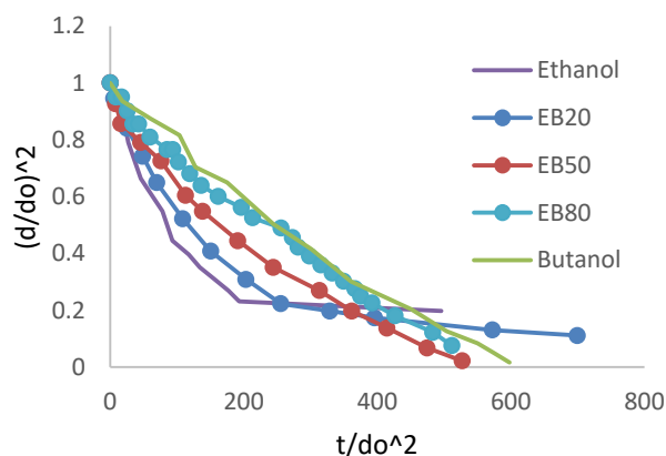
FIGURE 6. Evaporation Behaviour of Ethanol Butanol Blends
