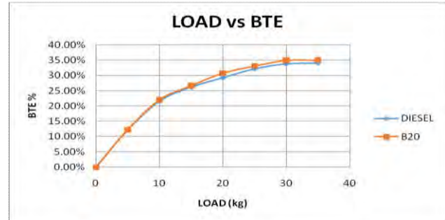
FIGURE 4. LOAD VERSES BRAKE THERMAL EFFICIENCY
