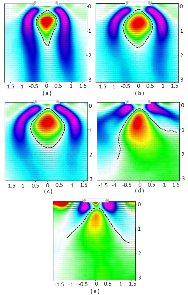
FIGURE 3. AXIAL VELOCITY CONTOURS SHOWING CTRZ BOUNDARY
