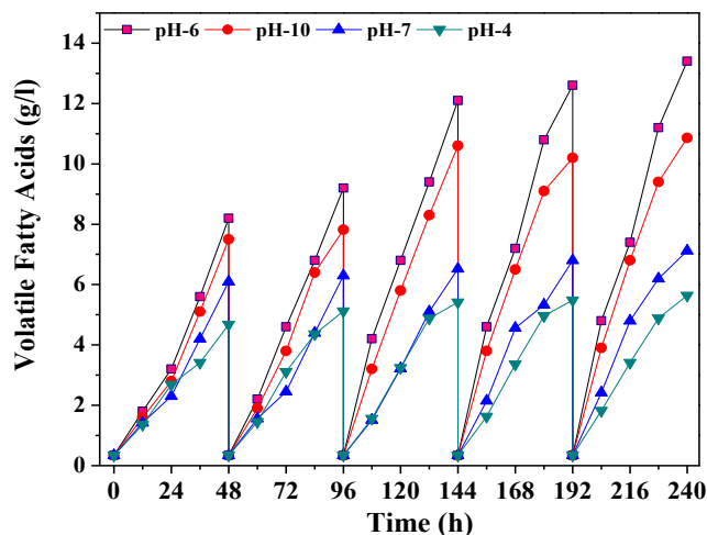
Fig 2: Volatile fatty acids concentration with the function of operation time
