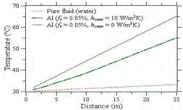
Figure 6 Fluid outlet temperature as a function of distance along the collector length.
