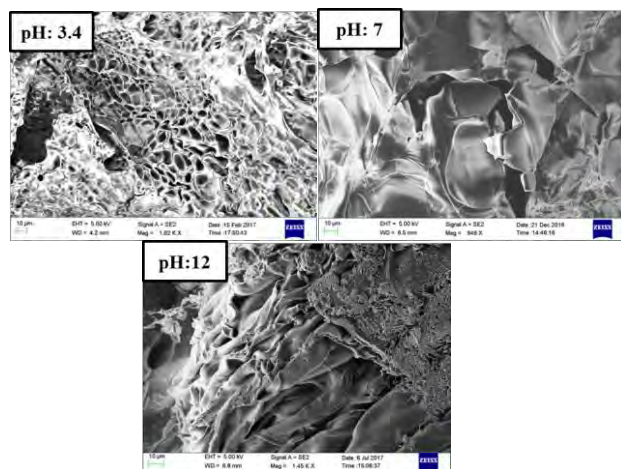
FIGURE 2: Characteristic SEM images of Poly (acrylic-co-vinylsulfonic) acid hydrogel at different pH solutions
