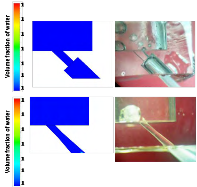
Figure 6: Absence of cavitation in sharp exit film cooling orifice and diverging film cooling orifice under high back pressure condition computational results (left column) and experimental results (right column)
