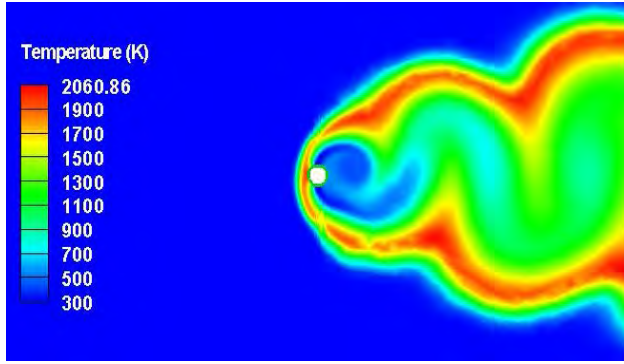
Fig. 4: Temperature contours for \phi=1
