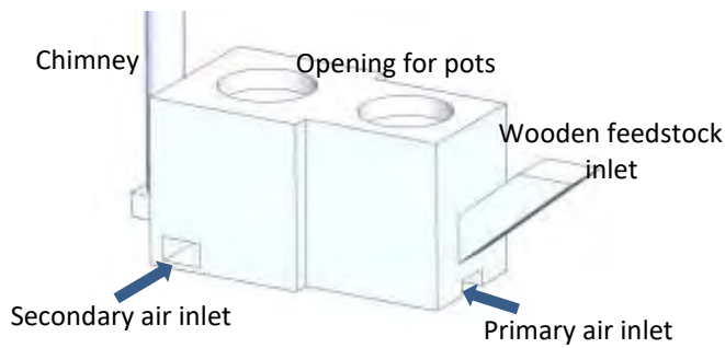
Figure 1a: External view of cook stove
