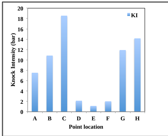
FIGURE 4: KNOCK INTENSITY AT POINTS A-H.
