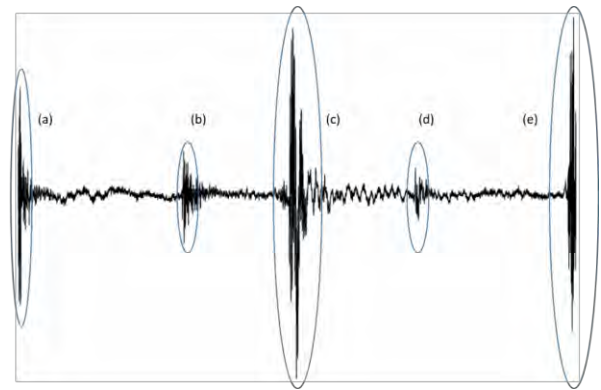
(a): Exhaust valve closes ( 4.5^\circ aTDC); (b): Inlet valve closes ( 35.5^\circ aTDC); (c) Combustion; (d) Exhaust valve opens ( 35.5^\circ bBDC); and (5) inlet valve opens ( 4.5^\circ bTDC)
