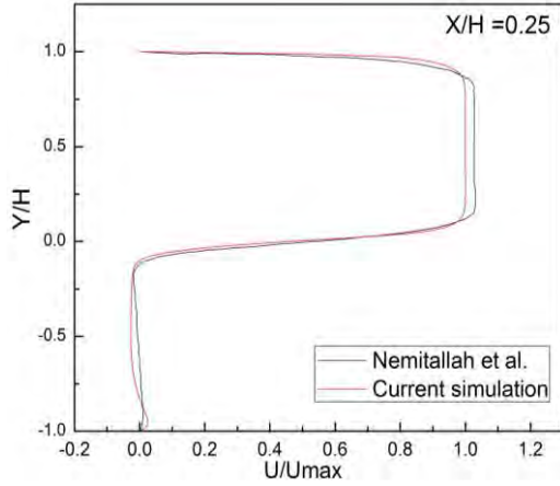
Fig 2: Velocity profile at normalized axial location X/H = 0.25 .
