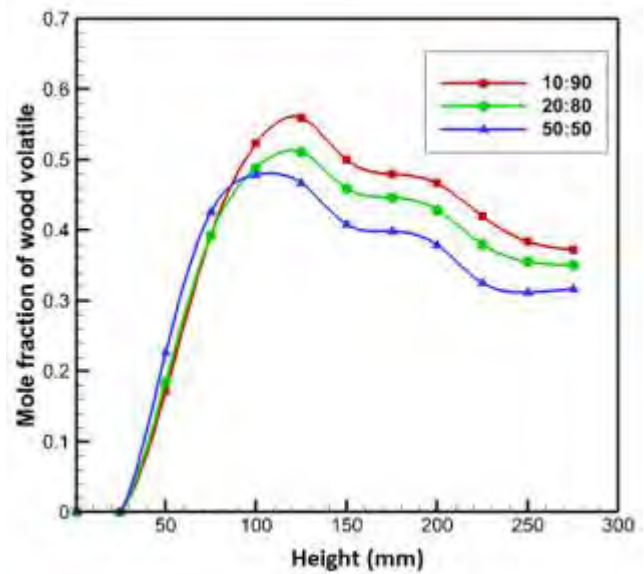
Figure 7b: Variation in mole fraction of wood volatile along the height of cook stove
