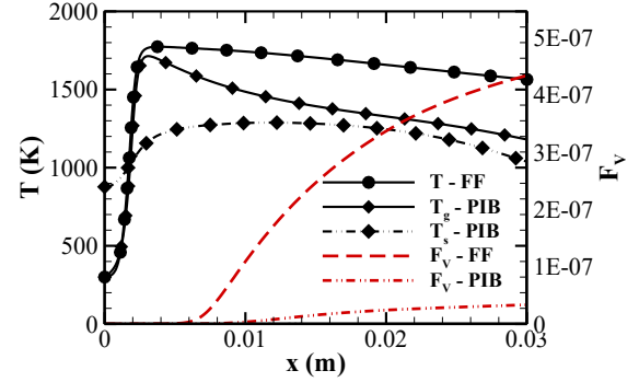
FIGURE 2. Comparisons of axial gas and solid-phase temperature profiles and soot volume fractions
