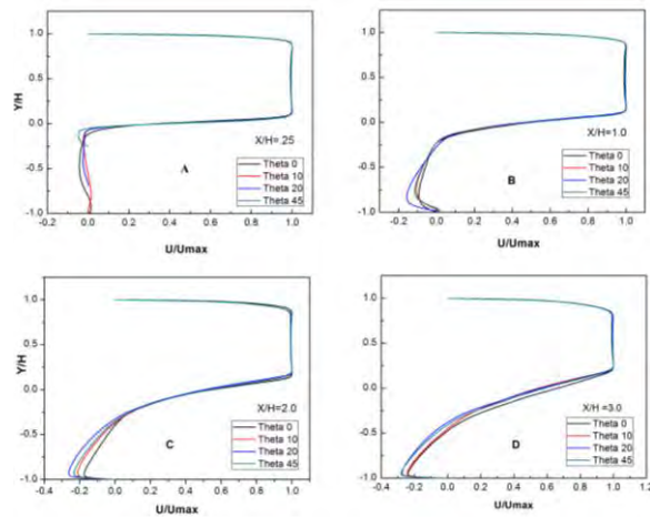
Fig 5: Average Velocity profile at different location of X/H (A) X/H= 0.25 (B) X/H = 1.0 (C) X/H= 2.0 (D) X/H = 3.0
