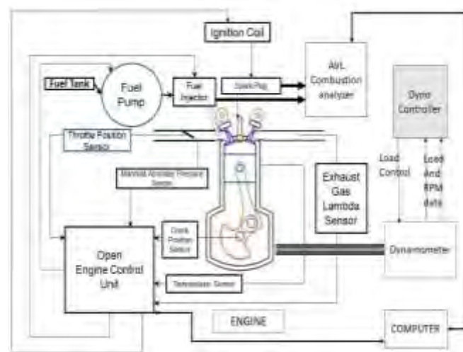
FIGURE 1: Schematic of the experimental setup for 4-stroke single cylinder methanol fuelled port fuel injection Spark ignition Engine
