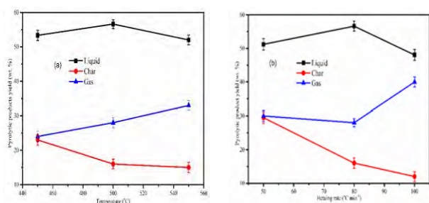
FIGURE 2. (A) EFFECT OF TEMPERATURE AND (B) EFFECT OF HEATING RATE ON PYROLYSIS
