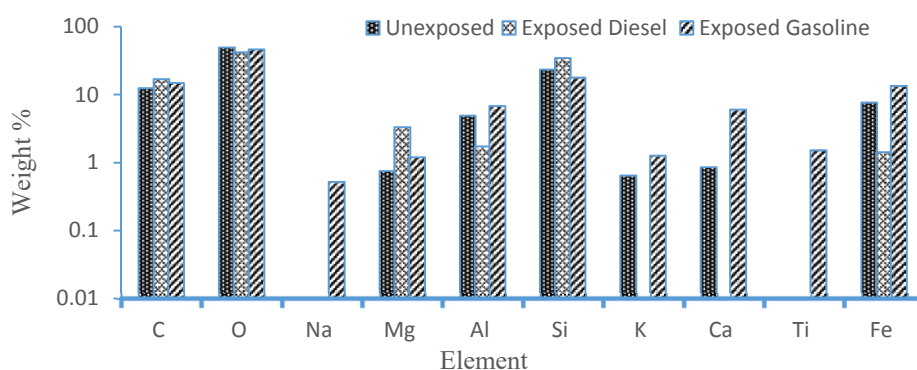
FIGURE 1. GRAPHICAL REPRESENTATION OF ELEMENTAL COMPOSITION OF UNEXPOSED, EXPOSED TO DIESEL AND EXPOSED TO GASOLINE SAMPLES OBTAINED BY ENERGY -DISPERSIVE X-RAY SPECTROSCOPY
