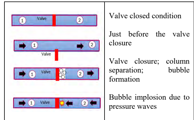
FIGURE 2. 1D REPRESENTATION OF NON-INERTIAL CAVITATION IN VALVES
