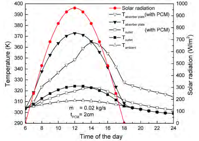
FIGURE 2. TRANSIENT TEMPERATURE VARIATION OF THE VARIOUS ELEMENTS OF FLAT PLATE SOLAR AIR HEATER WITH AND WITHOUT PCM.
