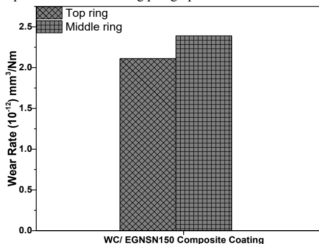
FIGURE 3. Wear rate of dual coating on engine piston ring after engine firing test.
