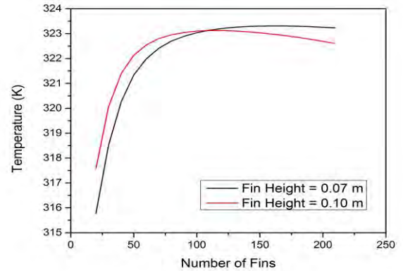
FIGURE 4: VARIATION OF OUTLET TEMPERATURE WITH NUMBER OF FINS FOR FIN THICKNESS t_1 = 0.003 m AND t_2 = 0.0015 m
