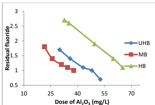
Fig.2: Comparative analysis of different variants of IPC v/s residual fluoride
