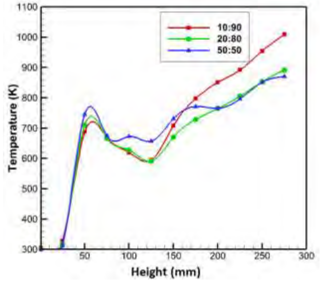
Figure 7a: Temperature variation along the height of cook stove
