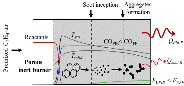
FIGURE 1. Soot growth process within PIB.
