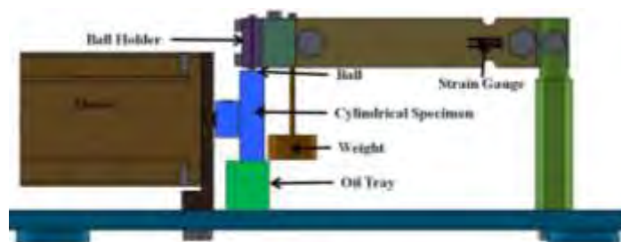
FIGURE 1. Ball-on-cylinder type tribometer.
