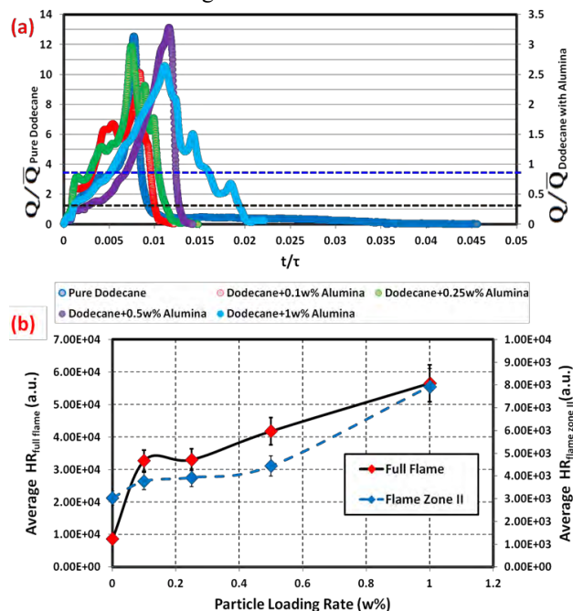
FIGURE 6 (a) Temporal history of normalised instantaneous heat release for all cases. (b) Average heat release (considering full and flame zone II) variation with PLR [6].
