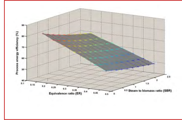
FIGURE 5 VARIATION OF ENERGY EFFICIENCY WITH ER AND SBR (T: 1000 K)
