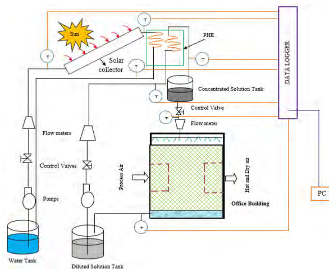
FIGURE 9. SCHEMATIC LINE DIAGRAM FOR THE EXPERIMENT.
