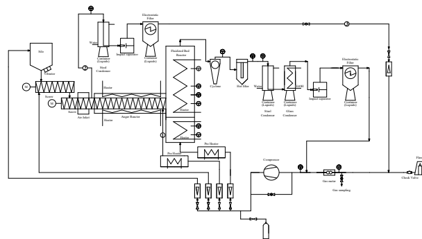
Figure 2. Schematic diagram of two-stage pyrolysis process
