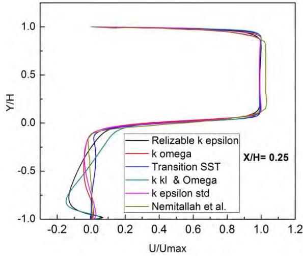
Fig 3: Velocity profile using various turbulence model at normalized axial locations at X/H = 0.25 .
