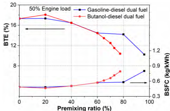
FIGURE 3. Effect of fuel premixing ratio on BTE and BSFC for gasoline/butanol-diesel dual fuel operation
