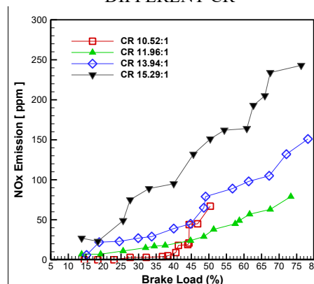
FIGURE 7. NO x EMISSION OF THE ENGINE AT DIFFERENT CR
