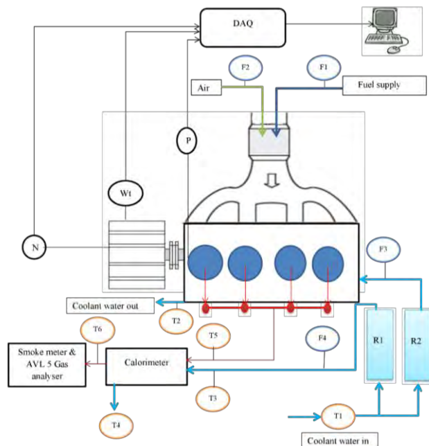
FIGURE 1. SCHEMATIC DIADRAM OF ENGINE
