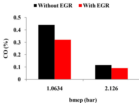
FIGURE 7: COMPARISON OF CO EMISSIONS WITH AND WITHOUT EGR
