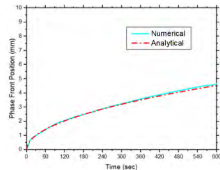
Figure 5. Comparison of phase front position of numerical vs. analytical method – Case 1.
