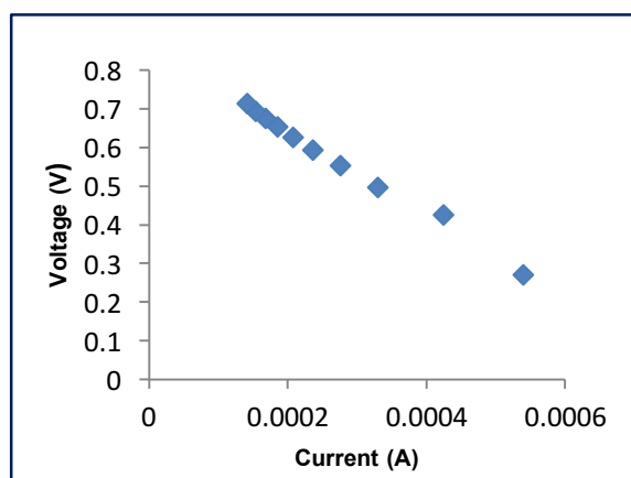
Fig.2.1 POLARIZATION BEHAVIOUR OF MFC WITH TE
