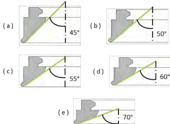
FIGURE 2. DESIGN OF FLARE GEOMETRY
