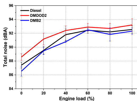
Figure 7. Total engine noise variation at different engine loads
