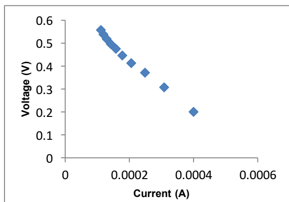
Fig.2.2 POLARIZATION BEHAVIOUR OF MFC WITH CE
