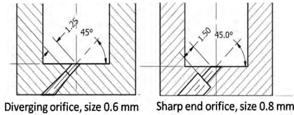
Figure1: Detail of orifice configuration
