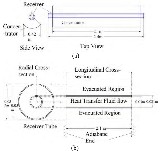
Figure 3. Schematic diagram of (a) PTC (b) receiver
