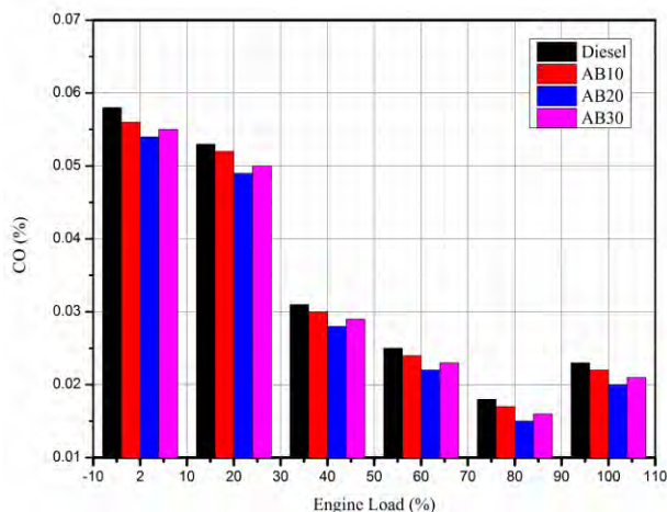
FIGURE 6. CO vs. engine load
