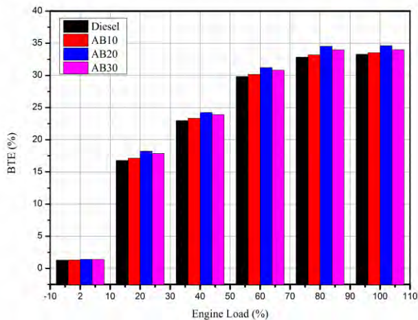
FIGURE 3. BTE vs. Engine load.
