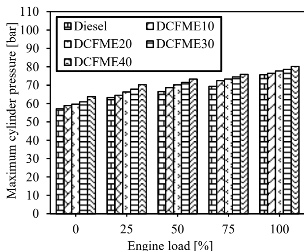
FIGURE 7 Variation of maximum cylinder pressure with load for diesel and DCFME blends.
