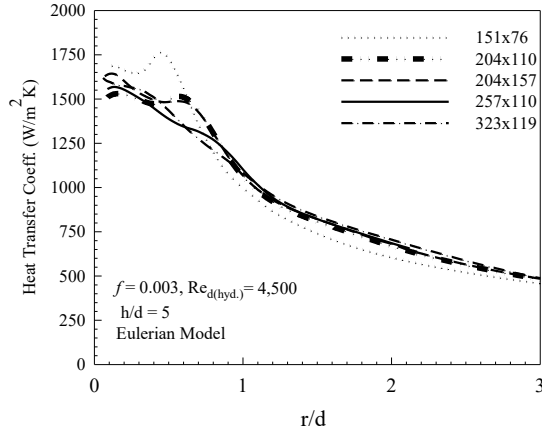
Figure 2:-Grid Independence Test
