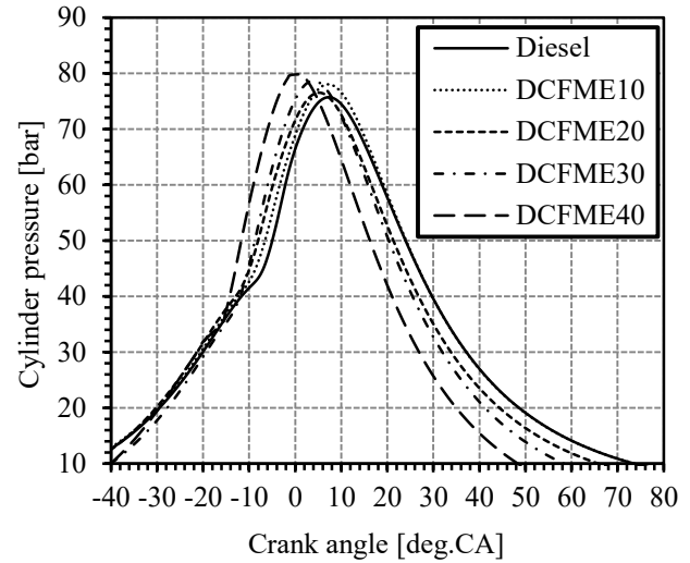
FIGURE 3 Variation of cylinder pressure for diesel and DCFME blends at full load.
