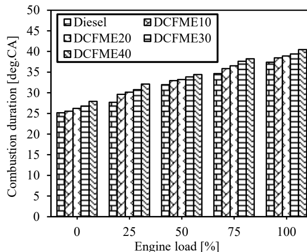
FIGURE 6 Variation of combustion duration with load for diesel and DCFME blends.
