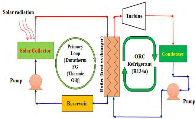
FIGURE 1. Schematic diagram of the primary and secondary loops of an ORC based medium temperature solar thermal power plant
