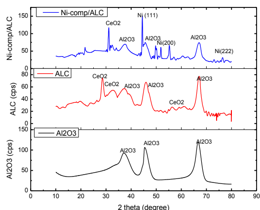
Figure. 2 Xray pattern of Support and catalyst
