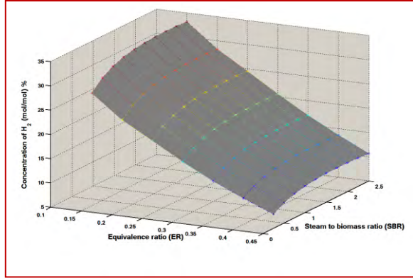
FIGURE 3 VARIATION OF H_2 CONCENTRATION WITH ER AND SBR (T: 1000 K)
