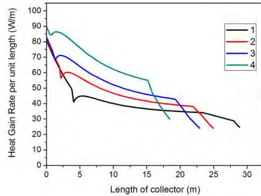
FIGURE 3. HEAT GAIN RATE ALONG THE LENGTH OF THE COLLECTOR FOR DIFFERENT REFRIGERANT MIXTURES
