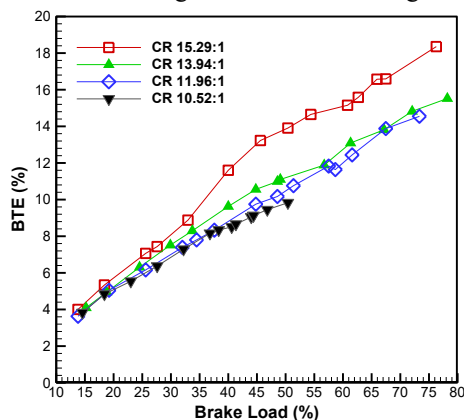
FIGURE 5. BRAKE THERMAL EFFICIENCY OF THE ENGINE AT DIFFERENT CR
