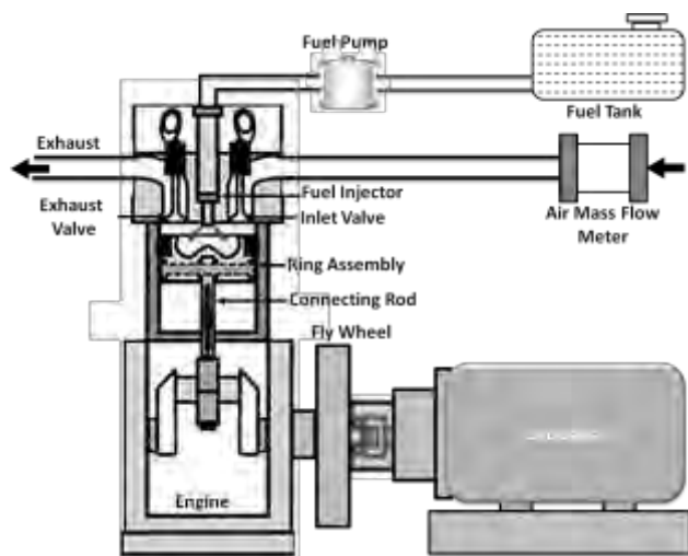
FIGURE 1. Schematic of test engine
