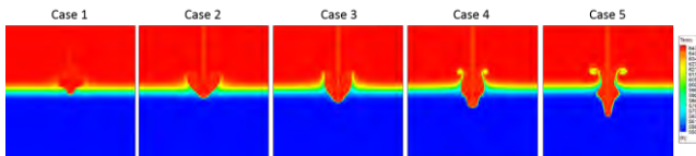
FIGURE 2. Contours of temperature at the instance of maximum penetration of disturbance fluid.
