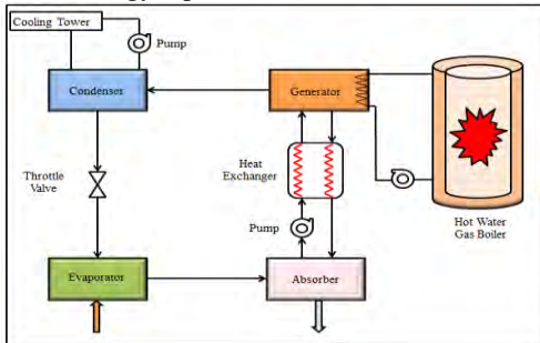
FIGURE 3. Schematic of Second Mode of Operation
