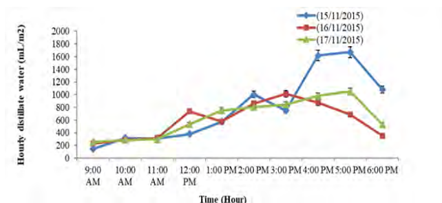
Fig. 4. Hourly variation of distilled output with time
