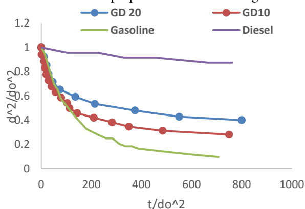
FIGURE 2. Evaporation Behaviour of Gasoline Diesel Blends
