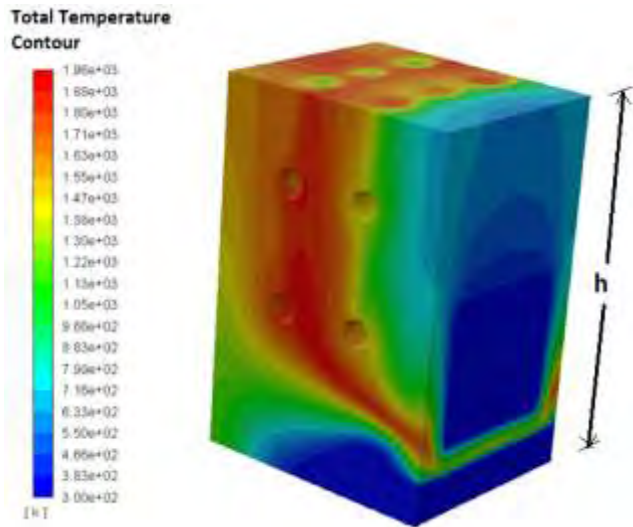
Figure 6: Temperature contours in combustion chamber
