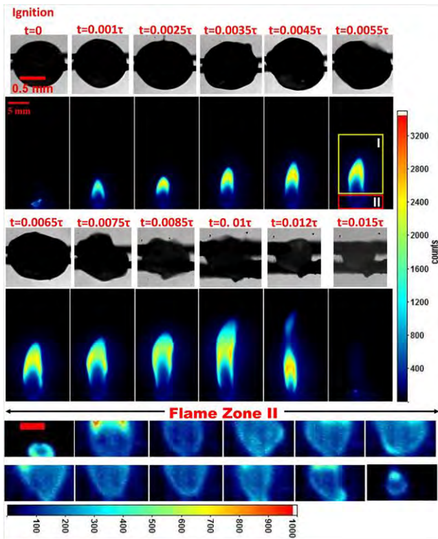
FIGURE 3 Simultaneous high speed imaging of shape oscillations and flame HR for PLR 1%. Flame zone II shows intense and localised fluctuations of the flame envelope due to ejection events. At the end stages, gelatinous mass is evidently present. The scale bar represents 2 mm [6].
