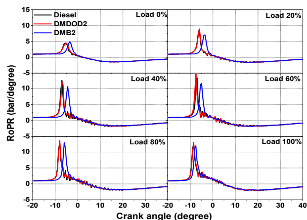
Figure 3. RoPR variation with CAD and engine load
