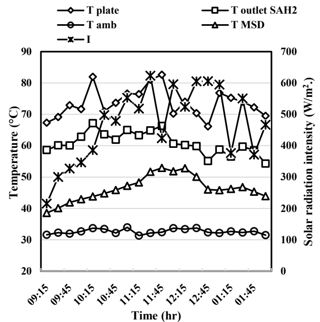
FIG.3 VARIATION OF TEMPERATURE AT DIFFERENT LOCATIONS OF MIXED MODE SOLAR DRYER AND SOLAR INTENSITY
