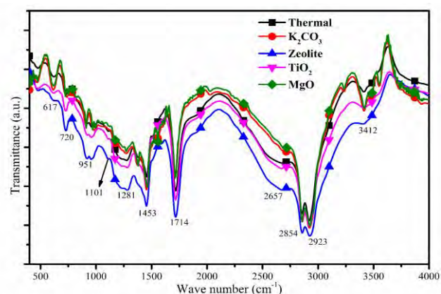
FIGURE 3. FTIR ANALYSIS OF THERMAL AND CATALYTIC PYROLYTIC LIQUID AT OPTIMIZED CONDITIONS.
