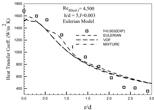
Figure 3:-Comparison of the Multiphase models for heat transfer results
