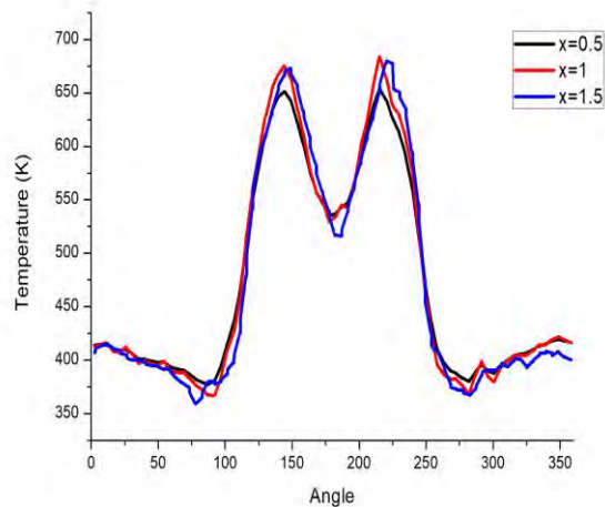
Figure 6. Temperature distribution on copper tube on angular direction
