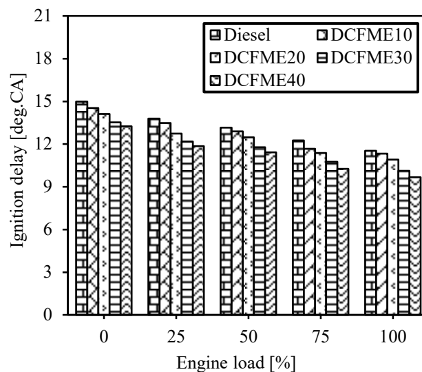
FIGURE 5 Variation of ignition delay with load for diesel and DCFME blends.
