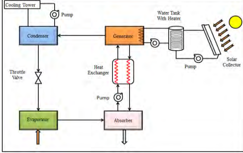
FIGURE 2. Schematic of First Mode of Operation
