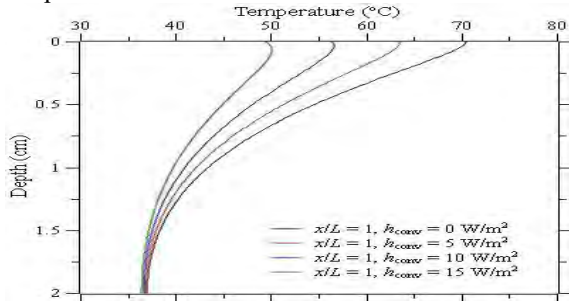
Figure 5 Temperature profile within the collector, at various convective heat transfer coefficients.
