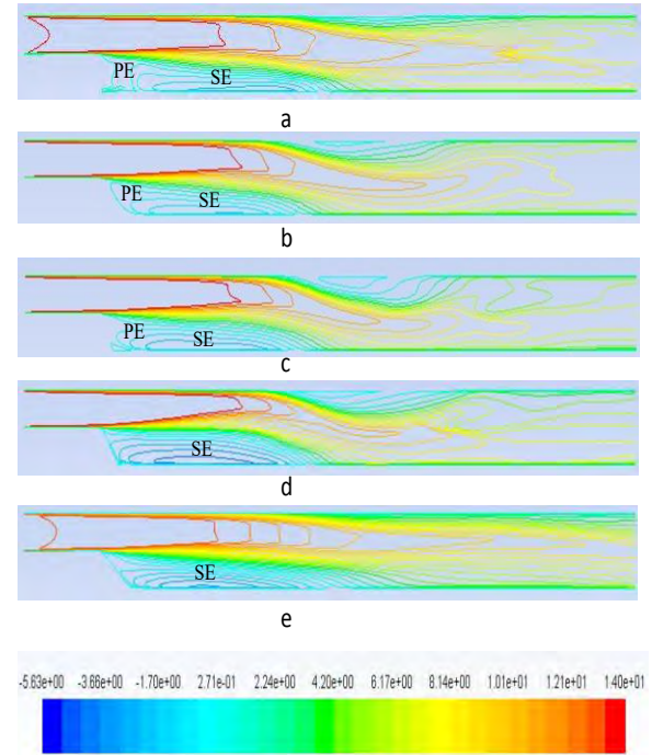
Fig 4: Contour plots of axial velocity for varied backward step angle for the dump combustor (a) \theta = 0^\circ (b) \theta = 10^\circ (c) \theta = 20^\circ (d) \theta = 30^\circ and (e) \theta = 45^\circ .
