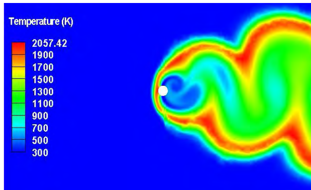
Fig. 5: Temperature contours for \phi=0.75
