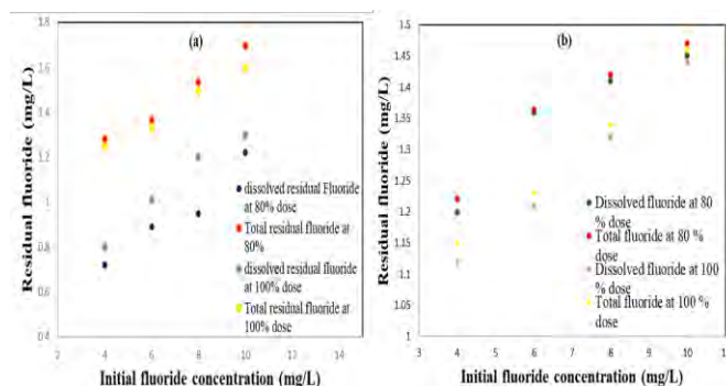
FIGURE 3 Total & dissolved fluoride of (a) alum and (b) PAC at 80% and 100% doses
