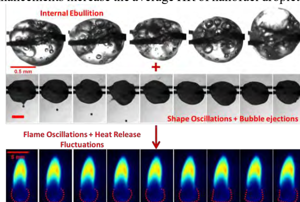
Figure 7 Pictorial representation of correlation of internal ebullition to shape oscillations and finally, to flame fluctuations.
