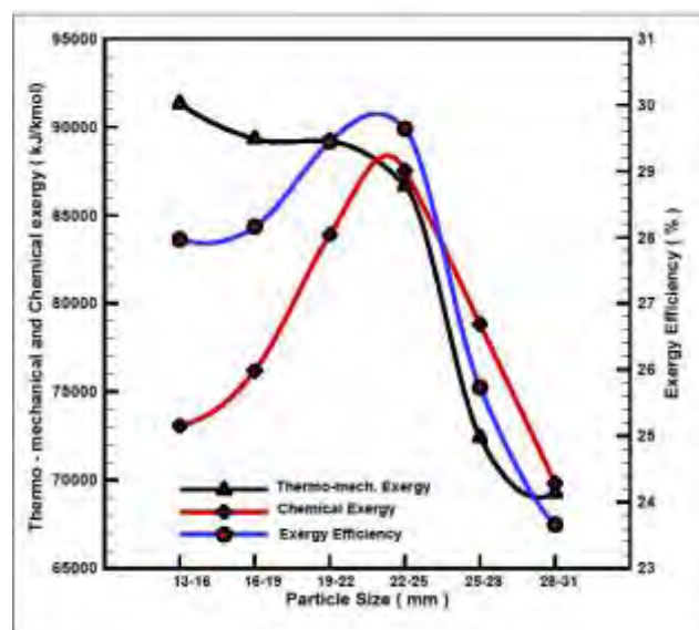
FIGURE 2. THE THERMO-MECHANICAL AND CHEMICAL EXERGY OF LIGNITE FOR DIFFERENT PARTICLE SIZES.
