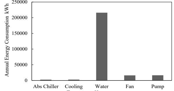
FIGURE 4. Energy Consumption for Solar Mode
