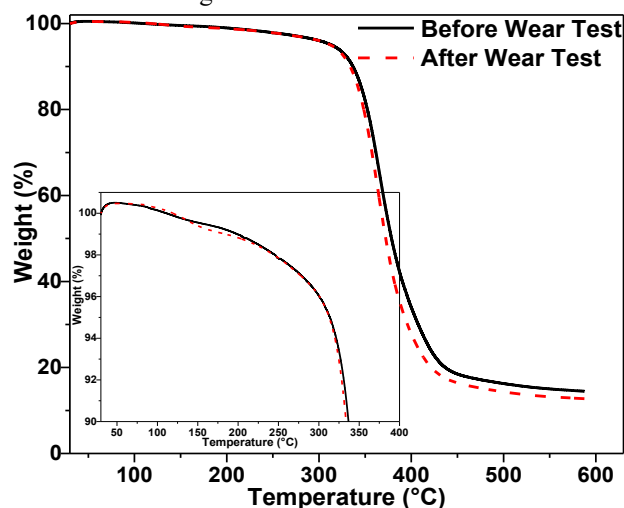
FIGURE 2. TGA of epoxy/ graphene/ SN150 composite before and after the engine test.
