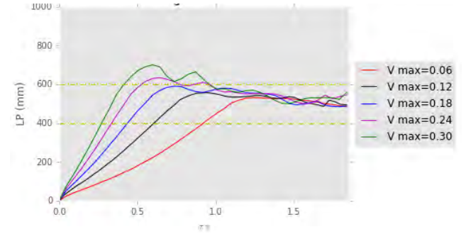
FIGURE 3. Track of inlet flow disturbance in TES system across all five cases
