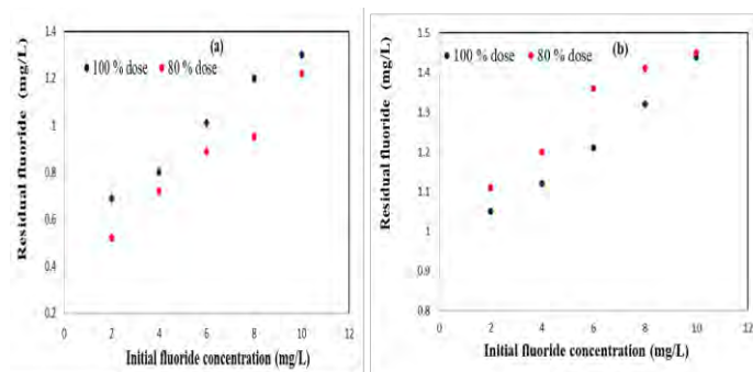
FIGURE 2 Comparative fluoride removal efficiency of (a) alum and (b) PAC at 80% and 100% doses in continuous mode
