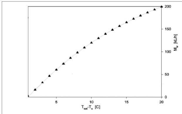
FIGURE 5. AMOUNT OF FRESHWATER PRODUCED AS A FUNCTION OF THE TEMPERATURE DIFFERENCE BETWEEN THE DEW POINT AND THE SURFACE TEMPERATURE AT AMBIENT TEMPERATURE T = 50^{\circ}\text{C} [1].
