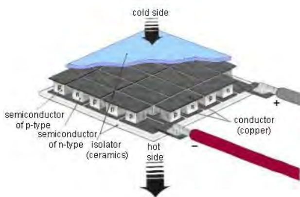
FIGURE 1: SCHEMATICS OF THE PELTIER DEVICE.
