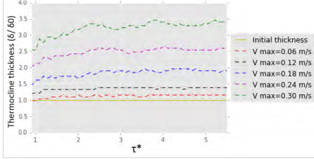
FIGURE 5. Transient variation of thermocline thickness across all five cases
