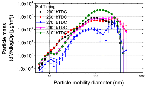
Figure 3: Particle size-mass distribution vs particle mobility
