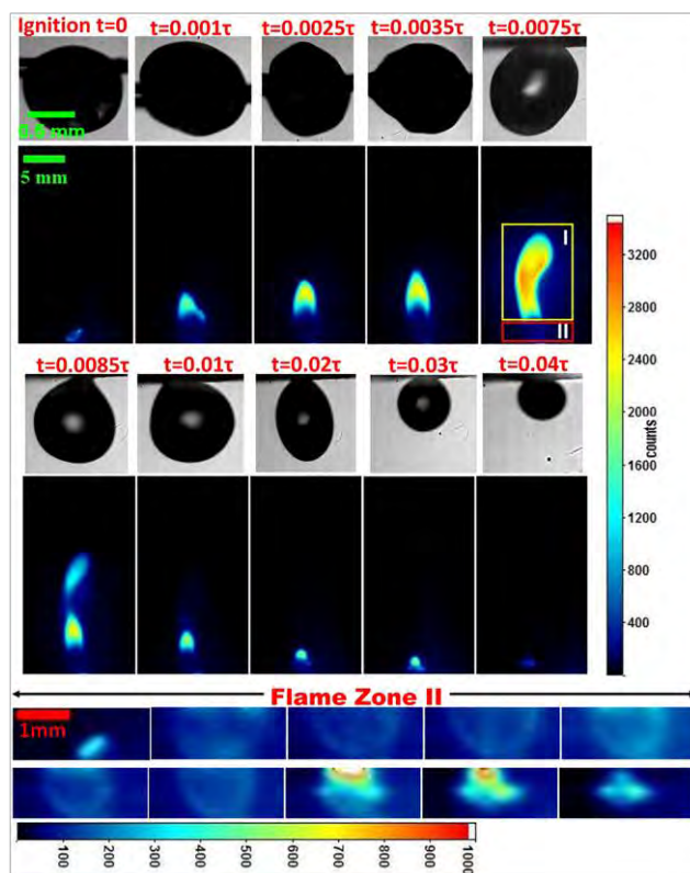
FIGURE 2 Simultaneous high speed imaging of surface oscillations and flame heat release for pure dodecane droplets at various time instants [6].
