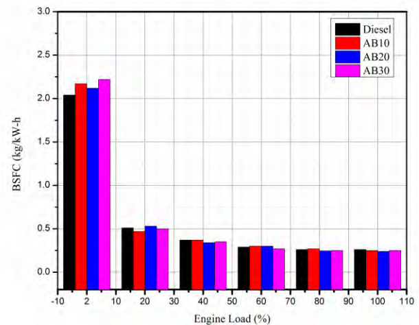
FIGURE 4. BSFC vs. Engine load
