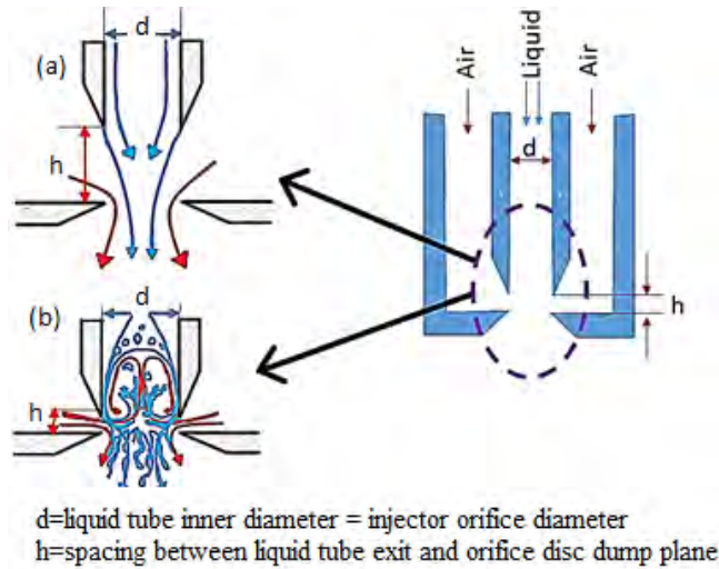
FIGURE 1. FLOW BLURRING TWIN FLUID ATOMIZATION CONCEPT (a) FLOW FOCUSING, (b) FLOW BLURRING BASED ON h/d RATIO.
