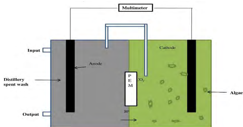
Fig 1. Experimental set used in this study
