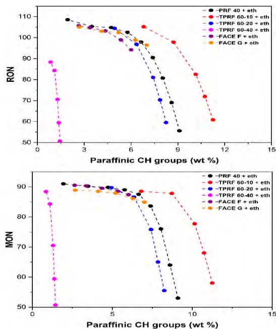
FIGURE 3. Effect of paraffinic CH groups on RON and MON of the blends
