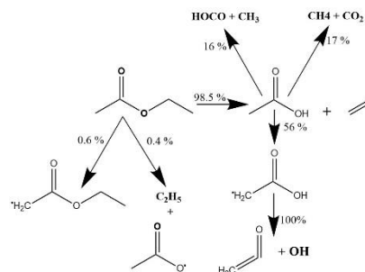
FIGURE 2: REACTION PATH ANALYSIS OF ETHYL ACETATE AT 10% OF FUEL CONVERSION TIME. P=15 BAR, 1200 K AND PHI =1.
