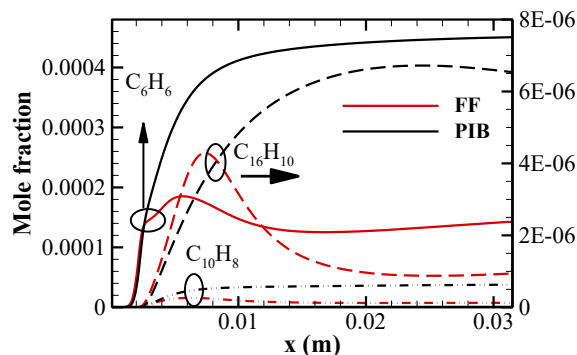
FIGURE 4. concentration profiles of major PAHs
