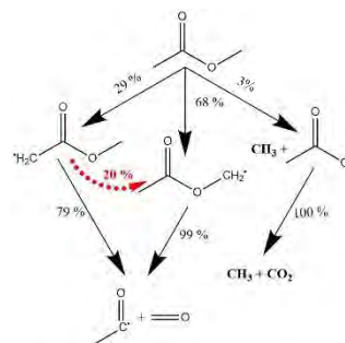
FIGURE 1: REACTION PATH ANALYSIS OF METHYL ACETATE AT 10% OF FUEL CONVERSION TIME. P=15 BAR, 1200 K AND PHI =1.
