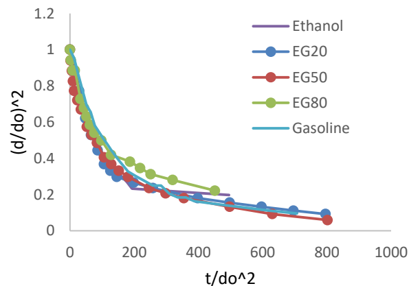
FIGURE 5. Evaporation Behaviour of Ethanol Gasoline Blends
