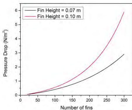
FIGURE 6: PRESSURE DROP V/S NUMBER OF FINS FOR FIN THICKNESS t_1=0.003 m AND t_2=0.0015 m.
