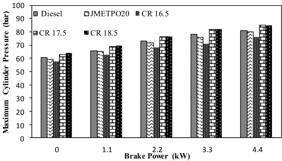
Variation of maximum cylinder pressure for test fuels at different compression ratio
