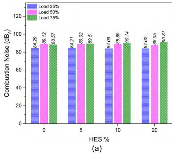
FIGURE 6. (a) Combustion noise measured using in-cylinder pressure transducer (b) Total noise as measured using microphone
