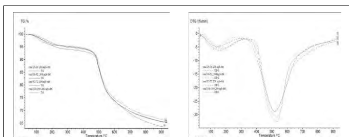
FIGURE 4. TG & DTG CURVES FOR HEATING RATE OF 200 K/MIN
