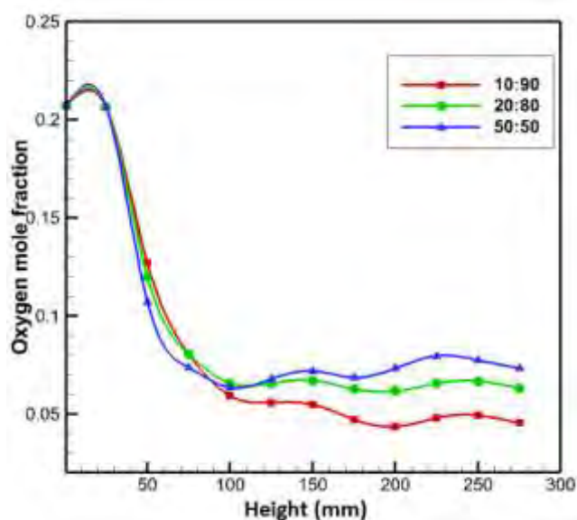
Figure 7d: Variation in mole fraction of oxygen along the height of cook stove
