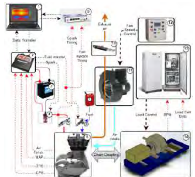
1- Computer interface, 2- Open-ECU, 3- Battery, 4- Laminar Flow Element, 5- Spark plug, 6- Fuel injector, 7- Fuel Tank, 8- Test engine, 9- Data acquisition system, 10-Exhaust tailpipe, 11- Intake air-filter, 12- Cooling fan controller, 13- Dynamometer controller, 14- Dynomerk eddy-current dynamometer
