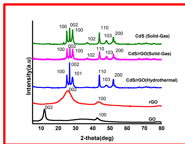
Figure2: XRD pattern of GO, rGO, CdS/rGO(hydrothermal), CdS/rGO (Solid-gas) and CdS(Solid-Gas)
