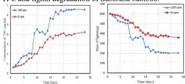
FIGURE 2: Effect of mixing on the TPC and lignin degradation of Bambusa bamboo in batch reactor.
