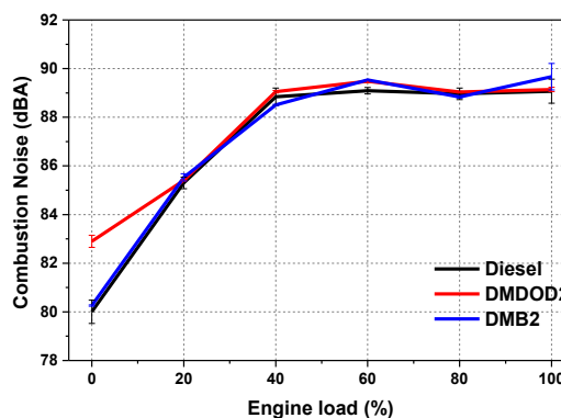
Figure 5. Variation of combustion noise with engine loads
