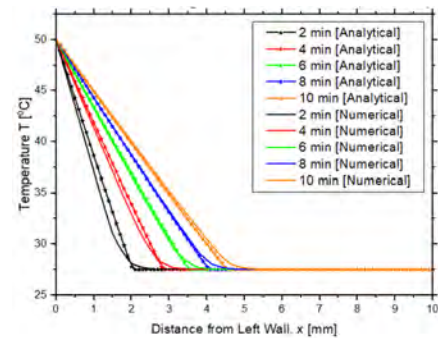
Figure 4. Comparison of temperature distribution of numerical vs. analytical method – Case1.
