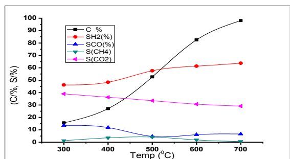
Fig 5. Effects of temperature on the conversion of acetic acid and Selectivities of the products. Experimental Conditions- S/C mol ratio 6.35:1; WHSV=1.26 h -1 ; P=1 atm
