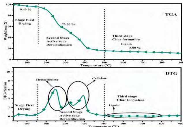
FIGURE 1. TGA AND DTG ANALYSIS OF RAW BIOMA
