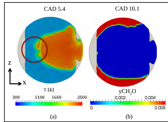
FIGURE 5: (a) END-GAS AUTO-IGNITION (CIRCLED), (b) FORMATION OF FORMALDEHYDE IN END-GAS PRE-IGNITION CYCLE.
