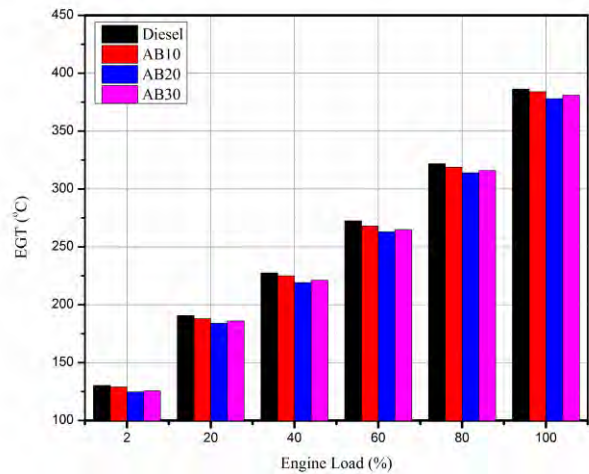
FIGURE 5. EGT vs. Engine load
