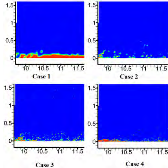
FIGURE 3. VOLUME OF FLUID FOR WATER AT DIFFERENT GRID SIZES
