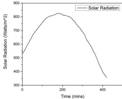
FIGURE 1: DATASOLAR RADIATION IN GUWAHATI REGION (26.11°N, 91.72°E).
