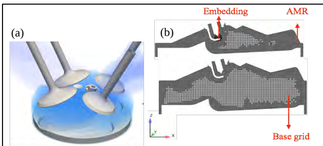
FIGURE 1: (a) GEOMETRY OF THE SI ENGINE, (b) MESH GENERATED FOR THE STUDY.
