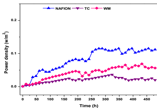
Fig. 1. Stable power density curves with respect to time in MFC N , MFC ML , MFC T
