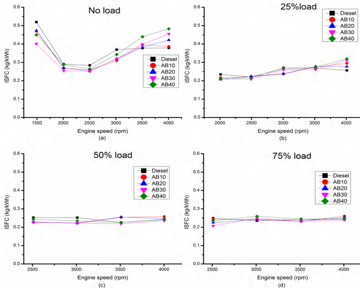
FIGURE 3. INDICATED SPECIFIC FUEL CONSUMPTION
