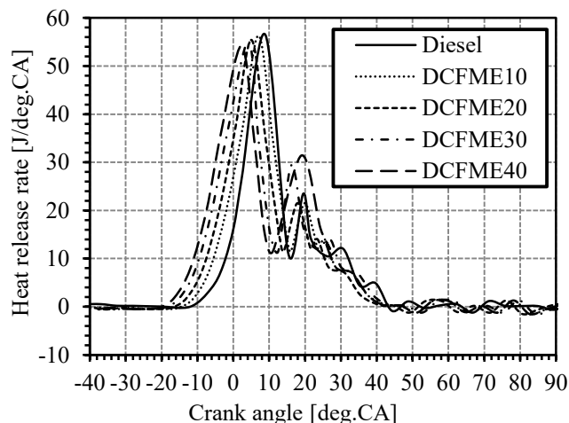
FIGURE 4 Variation of heat release rate for diesel and DCFME blends at full load.
