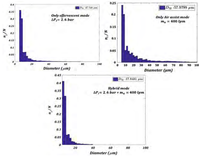
FIGURE 1. Drolpet distribution and SMD at various conditions
