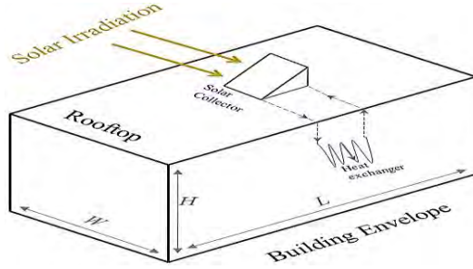
Figure 2 Schematic of the building envelope, showing the rooftop solar collector as well as the heat exchanger for space heating.
