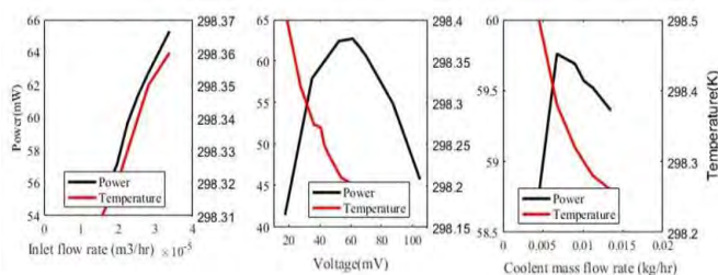
FIGURE 2. STEADY STATE PROFILE OF THE POWER AND TEMPERATURE OF THE CELL WITH MANIPUALTED VARIABLES
