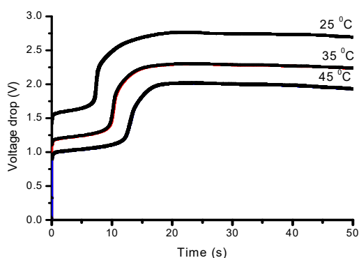
Fig.2 Chronopotentiometric curves for CMV membrane at 20.23 mA/cm 2 applied current densities in 0.10 M NaCl.
