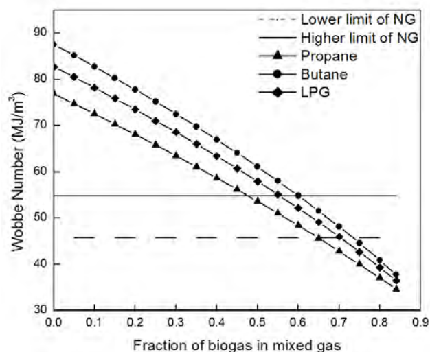
FIGURE 1. WOBBE NUMBER TO BIOGAS PERCENTAGE
