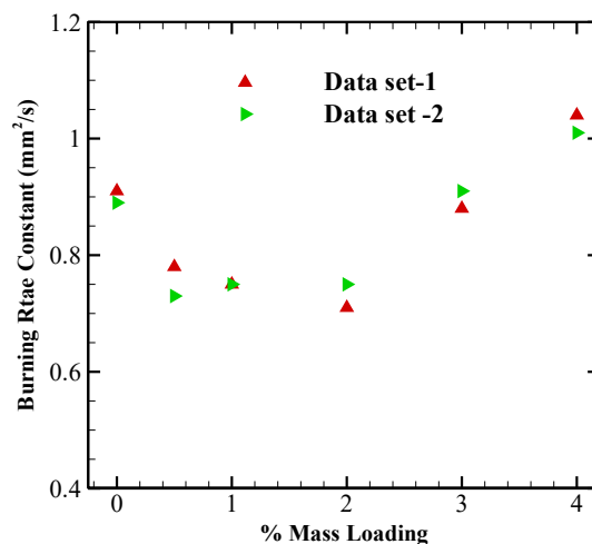
Figure-5 Variation of burning rate constant with % mass loading of ANP
