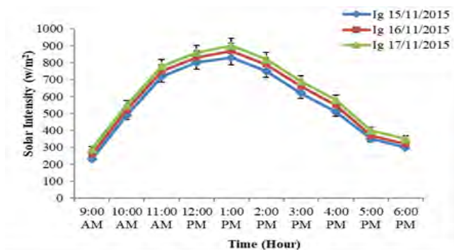
Fig.3 Variation of solar radiation with time
