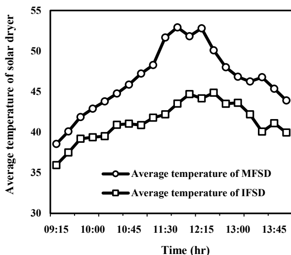
FIG.4. VARIATION OF AVERAGE TEMPERATURE INSIDE THE MFSD AND IFSD WITH DRYING TIME.
