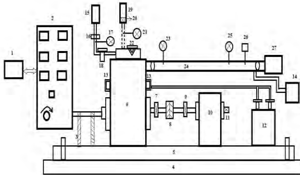
FIGURE 2 Schematic diagram of the experimental setup. 1. Data acquisition system, 2. Digital display unit, 3. Insulated cable box, 4. Engine bed, 5. Base frame vibration absorber, 6. Single cylinder CI engine, 7. Crank angle sensor, 8. Flywheel coupling, 9. Speed sensor, 10. Eddy current dynamometer, 11. Load cell, 12. Water lever controller, 13. Pressure sensor with water cooling arrangement, 14. Exhaust gas analyzer, 15. Fuel tank, 16. Filter, 17. Fuel flow sensor, 18. Fuel pump, 19. Air box, 20. Pressure transducer, 21. Air flow sensor, 22. Fuel injector, 23. K-type thermocouple 1, 24. Exhaust gas calorimeter, 25. K-type thermocouple 2, 26. Exhaust gas sensor, 27. Smoke meter.
