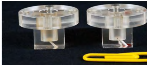
Figure 3: Diverging orifice (left) Sharp exit orifice (right)
