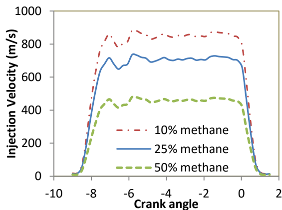
FIGURE 3. INJECTION VELOCITY WITH METHANE PERCENTAGE
