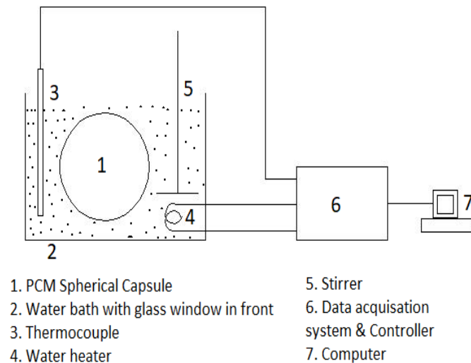
FIGURE 1. EXPERIMENTAL WATER BATH SETUP FOR SPHERICAL PCM CAPSULE
