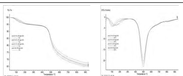
FIGURE 2. TG & DTG CURVES FOR HEATING RATE OF 100 K/MIN.
