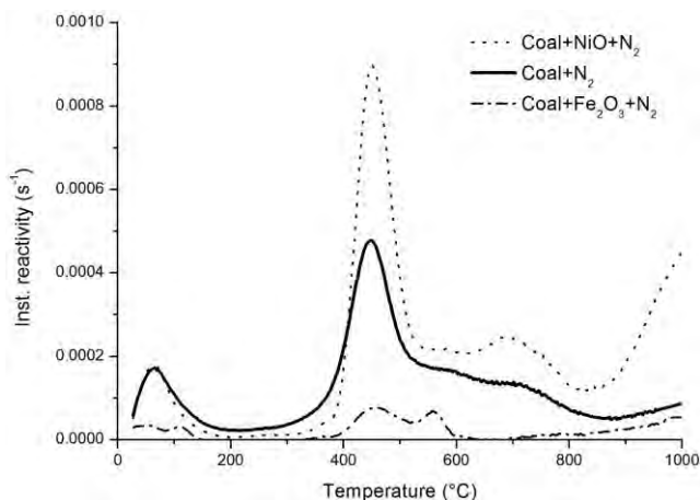
FIGURE 1. Instantaneous reactivity of low ash coal with \text{Fe}_2\text{O}_3 and \text{NiO} in \text{N}_2 atmosphere
