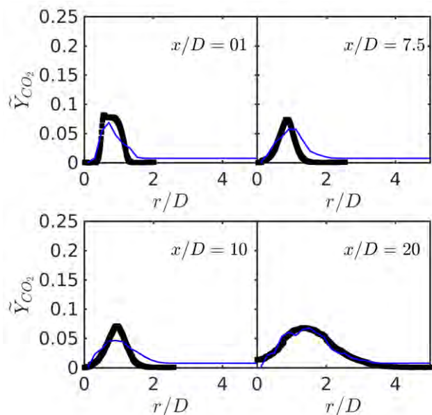
Figure 2: Radial profiles of CO 2 mass fraction at different axial locations.
