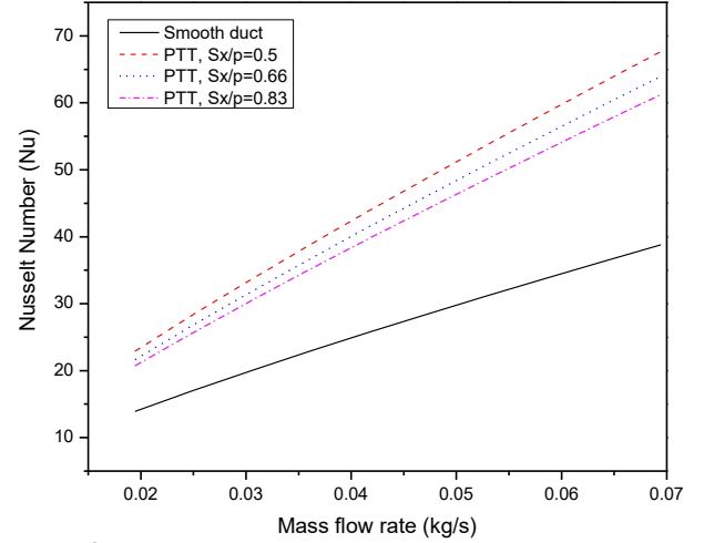
FIG. 2 VARIATION OF NUSSULT NUMBER WITH MASS FLOW RATE.
