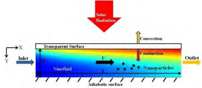
Figure 3 Schematic of the solar collector using nanoparticles.
