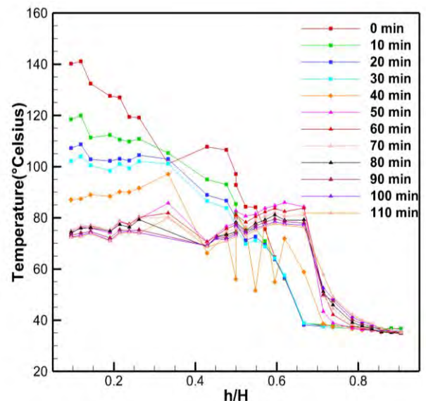
Figure 3. Profile of the thermocline using HITHERM-600.
