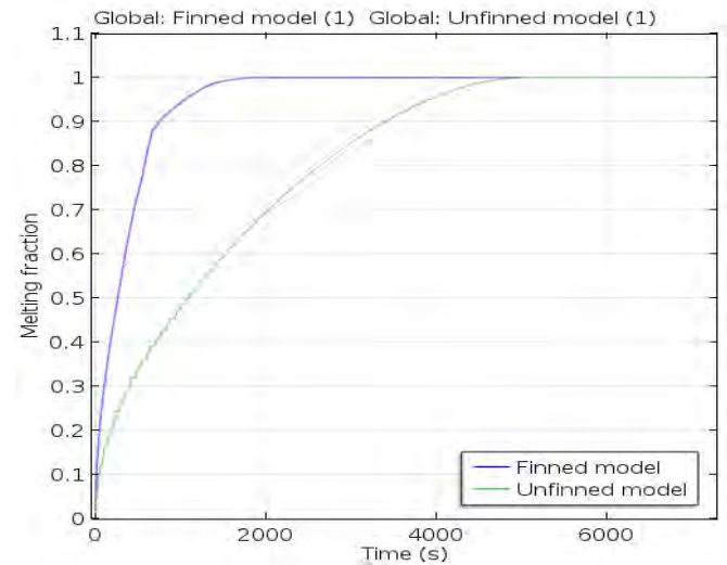
FIGURE 5. MELT FRACTION VS TIME (S) FOR UNFINNED AND FINNED PCM CAPSULE
