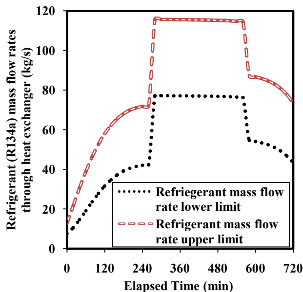
FIGURE 5. Variation of the ORC refrigerant (R134a) mass flow rate with changing temperature of the heat transfer fluid Duratherm FG ( T_{HTF} )
