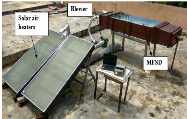
Fig.2 Pictorial view of MFSD setup
