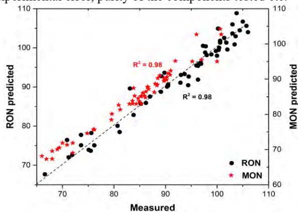
FIGURE 4: Comparison of experimental and predicted RON and MON values
