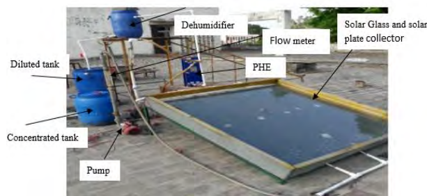
FIGURE 8. PHOTOGRAPHIC VIEWS OF EXPERIMENTAL SET-UP.
