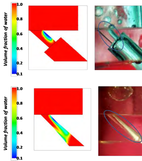
Figure 5: Cavitation observed in sharp exit film cooling Orifice and diverging film cooling orifice under 1atm back pressure condition computational results (left column) and experimental results (right column)
