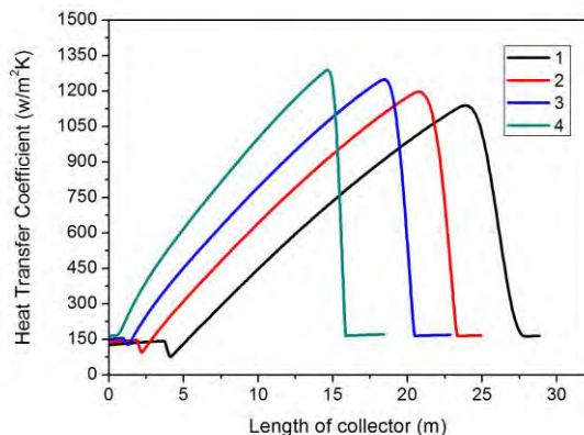
FIGURE 4. HEAT TRANSFER COEFFICIENT ALONG THE LENGTH OF THE COLLECTOR FOR DIFFERENT REFRIGERANT MIXTURES
