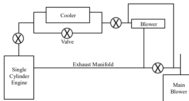
FIGURE 1: EGR LOOP
