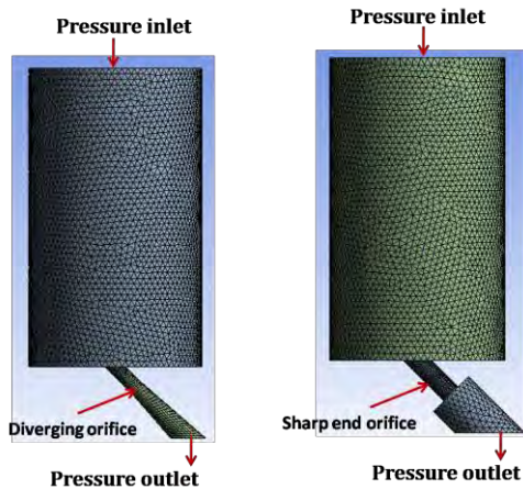
Figure 2: Mesh and boundary conditions
