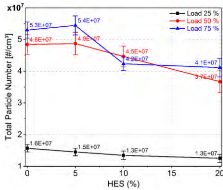
Figure 3 Effect of HES on the total particulate number (PN).
