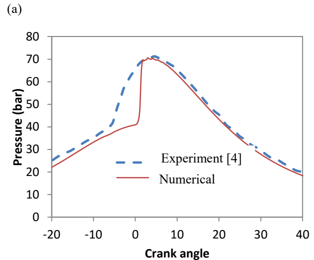
FIGURE 1. (a) PRESSURE TRACE FOR DIFFERENT GRID SIZE (b) COMPARISON OF PRESSURE WITH EXPERIMENTAL DATA FOR VALIDATION.
