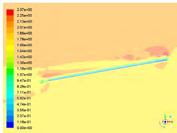
FIGURE 4: Velocity magnitude (m/s) contours around the PV module in z-plane
