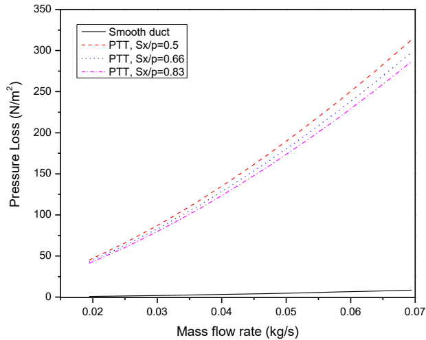
FIG. 4. EFFECT OF MASS FLOW RATE ON THE PRESSURE LOSS ACROSS THE DUCT.
