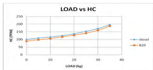
FIGURE 6. LOAD VERSES HYDROCARBON EMISSION
