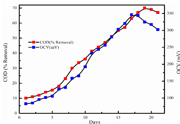
Fig 3. Relation between COD (% removal) and OCV (mV)
