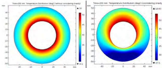
Figure 8. Comparison of temperature distributions -case 3.
