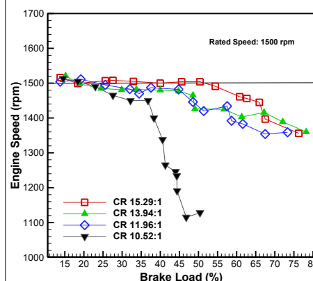
FIGURE 3. SPEED DEVELOPED BY THE ENGINE AT DIFFERENT COMPRESSION RATIOS
