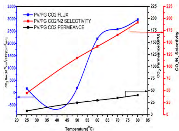
FIGURE 4: Effect of temperature on \text{CO}_2 permeance(GPU),and \text{CO}_2/\text{N}_2 selectivity for pure PVA/PG PM at feed absolute pressure= 1.5\text{ atm} , sweep absolute pressure= 1\text{ atm} , and water flow rates = 0.03/0.04\text{ ml/min} (feed/sweep).
