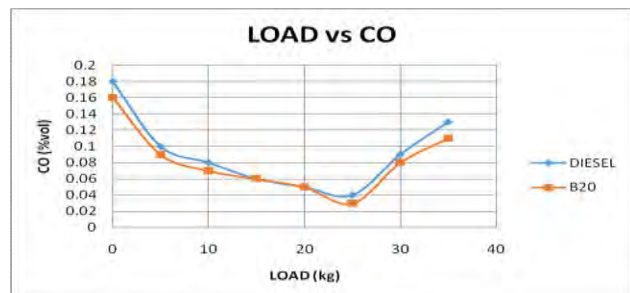
FIGURE 7. LOAD VERSES CARBON MONOXIDE EMISSION
