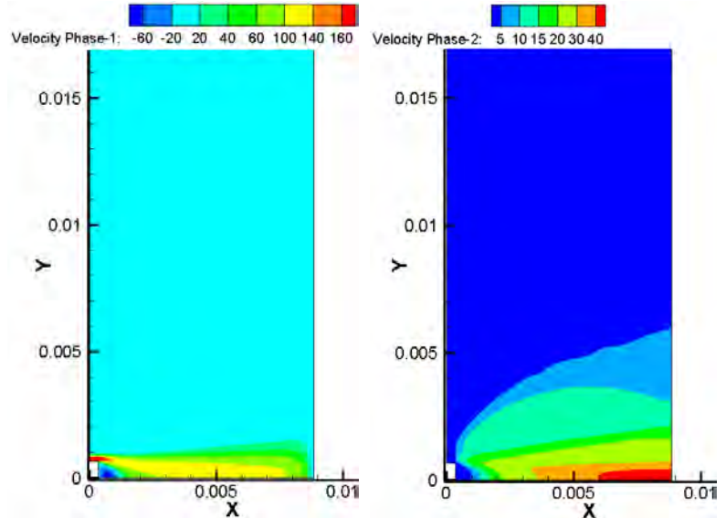
Figure 4:-Contours of Velocity for air and water.
