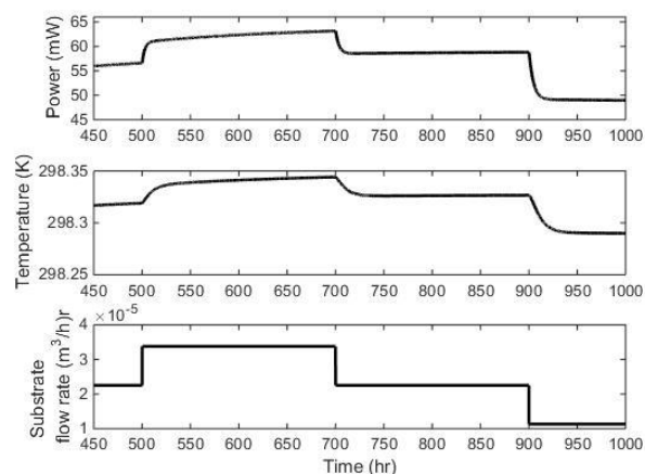
FIGURE 3. DYNAMIC RESPONSE OF SUBSTRATE FLOW RATE ON THE POWER AND TEMPERTURE
