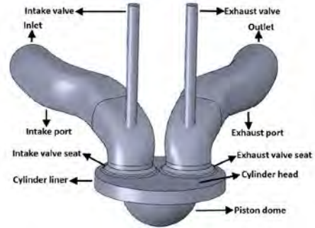
FIGURE 1. COMPUTATIONAL FLUID DOMAIN
