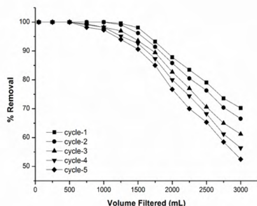
FIGURE 1. REMOVAL EFFICIENCY OF MODIFIED UF-MEMBRANE FOR CONSECUTIVE 5 CYCLES USING DICLOFENAC SODIUM AQUEOUS SOLUTION AT PH 7.5 AND TEMPERATURE 30°C
