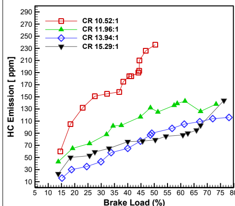
FIGURE 6. HC EMISSION OF THE ENGINE AT DIFFERENT CR
