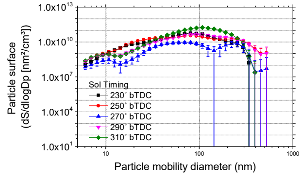
Figure 4: Particle surface area distribution vs particle mobility diameter (nm)
