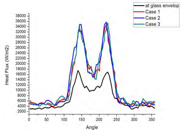
Figure 5. Solar energy flux distribution on the absorber tube with different case
