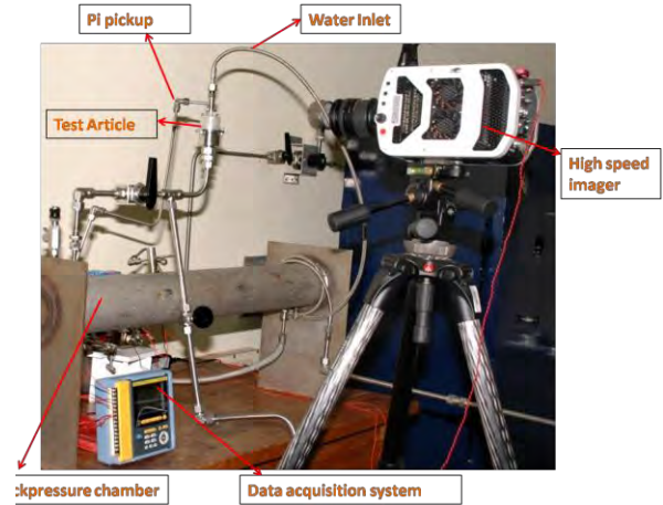
Figure 4: Complete experimental set up
