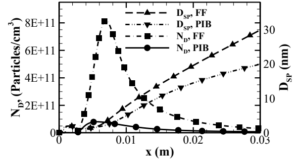
FIGURE 3. Comparisons of particle number densities and soot diameters as a function of burner distance
