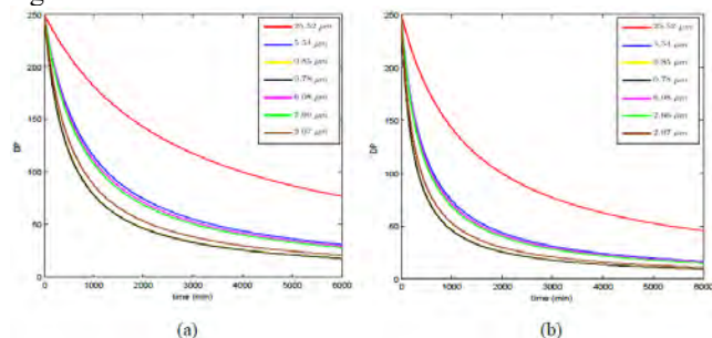
FIGURE 6: Effect of particle size on DP under non-competitive inhibition obtained from model simulation for the initial cellulose concentration of (a) 20 mg/ml (b) 10 mg/ml.
