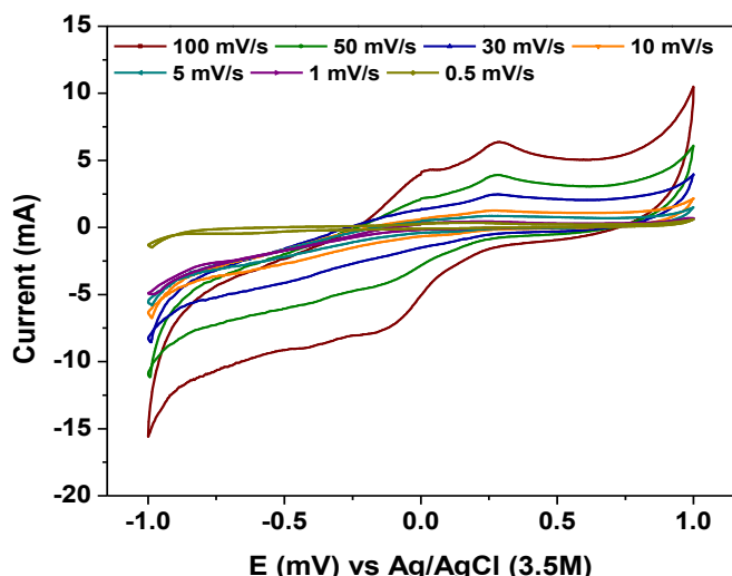
Fig 1: Cyclic voltammogram profiles depicting the photobacteria and cyanobacteria synergistics
