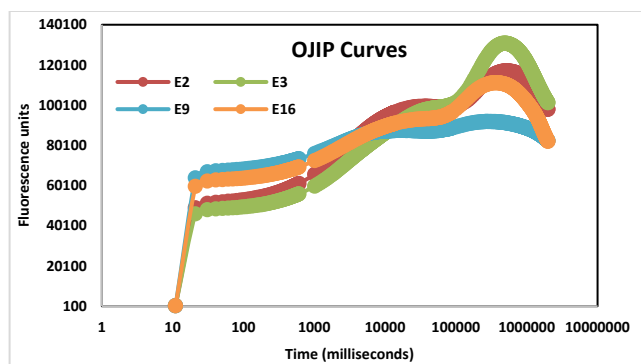
Fig 1: Photosynthetic efficiency in growth phase measured OJIP curves
