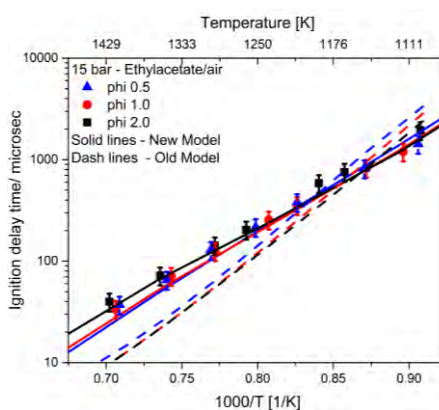
FIGURE 5: COMPARISON OF ETHYL ACETATE IGNITION DELAY DATA WITH PROPOSED MODEL AND MODEL BY WESTBROOK ET AL.
