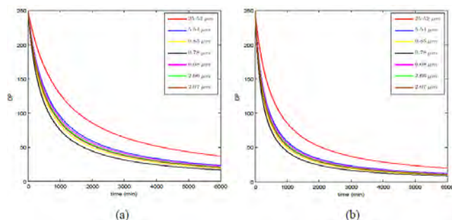
FIGURE 5: Effect of particle size on DP under competitive inhibition obtained from model simulation for the initial cellulose concentration of (a) 20 mg/ml (b) 10 mg/ml.
