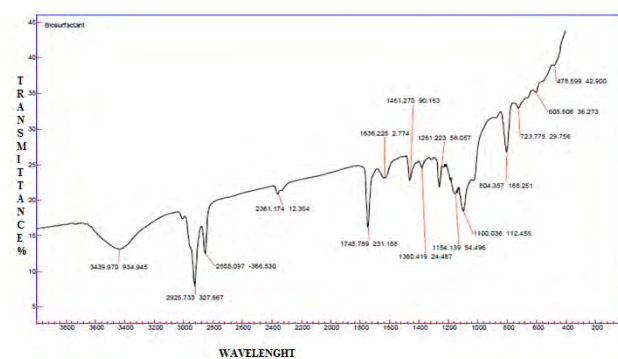
FIGURE 2: FT-IR ANALYSIS
