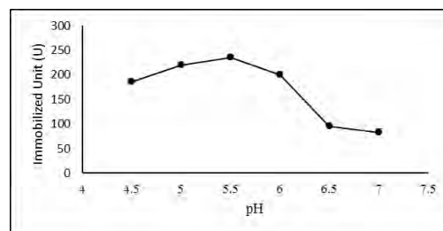
FIGURE. 2- OPTIMISATION OF pH
