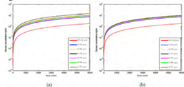
FIGURE 3: Effect of particle size on glucose yield under competitive inhibition obtained from model simulation (eqn. 9) for the initial cellulose concentration of (a) 20 mg/ml and (b) 10 mg/ml.
