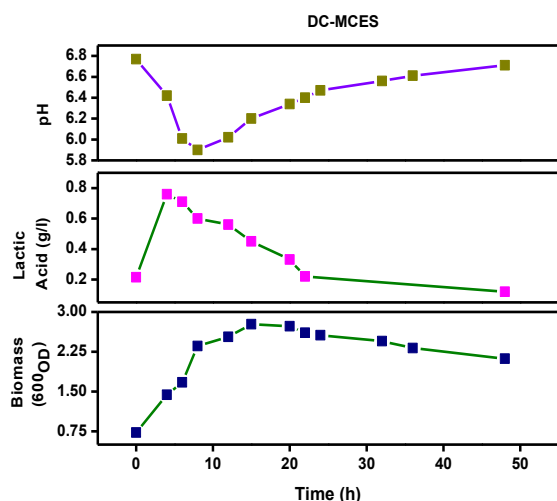
FIGURE 2: The profile specifies pH change, lactic acid production and biomass with respect to time for Closed circuit operation for Double chamber MCES
