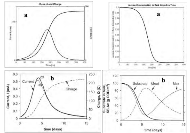
FIGURE 1. QUALITATIVE VALIDATION OF BATHCH MODEL WITH LITERATURE, A) TRENDS FROM MODEL SIMULATION, AND B) TRENDS FROM LITERATURE
