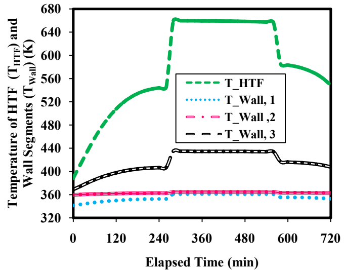
FIGURE 4. Variation of temperature of the wall segments ( T_{wall,1} , T_{wall,2} , T_{wall,3} ) with the changing temperature of the heat transfer fluid Duratherm FG ( T_{HTF} )
