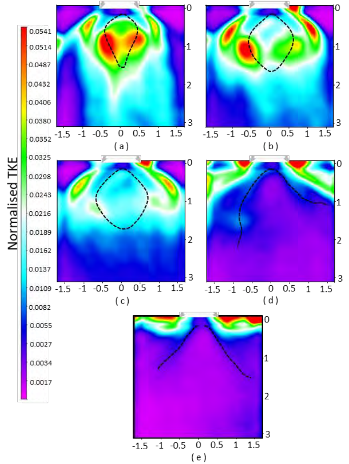
FIGURE 4. NORMALIZED TKE CONTOURS a) CASE 1 b) CASE 2 c) CASE 3 d) CASE 4 e) CASE 5
