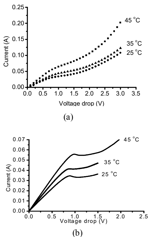
Fig.1 Effect of temperature on (a) current-voltage curves and (b) LSV curves for CMV membrane in 0.10 M NaCl.
